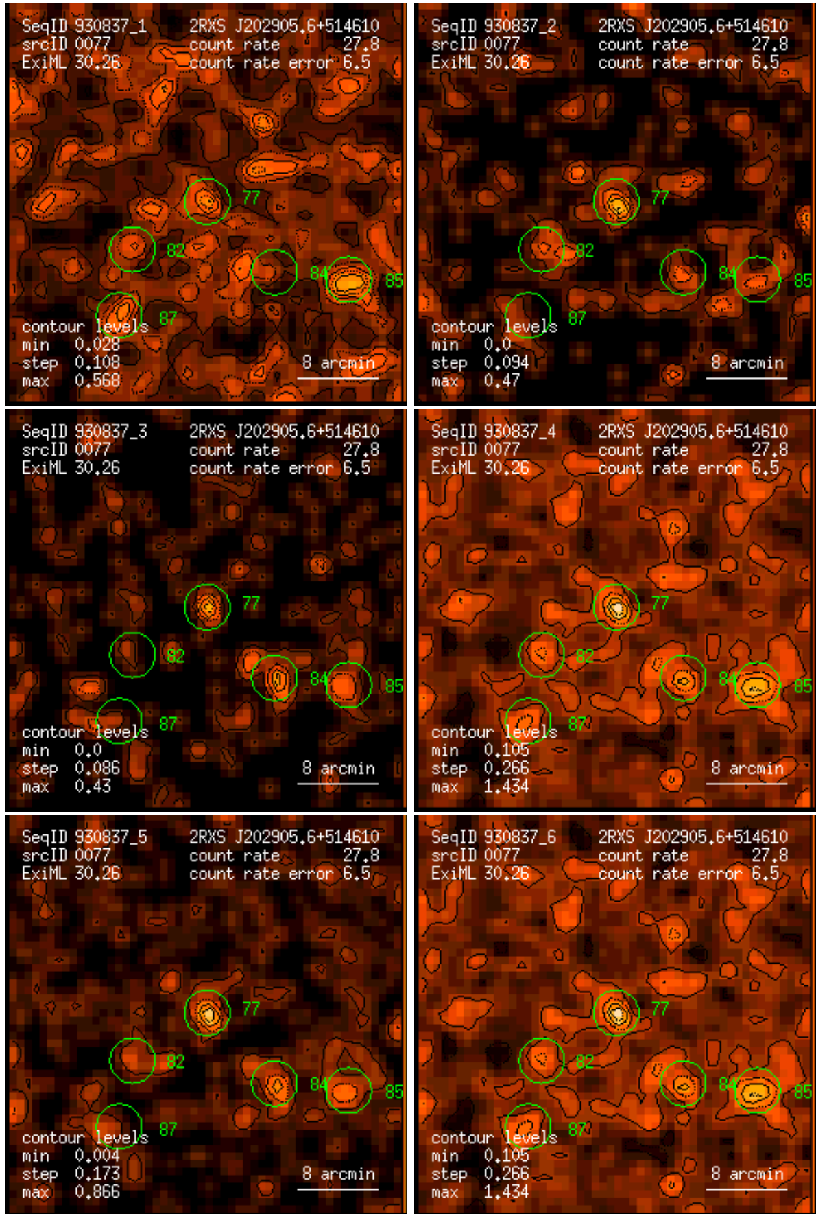
Figure 77: RASS 930837: detection 0077: band rate images, Gaussian filter: (1) PSPC channels 11 – 41, (2) 52 – 90, (3) 91 – 201, (4) 11 – 235, (5) 52 – 201, (6) 11 – 201. Broad band rates in counts/ks. Band rate contour levels in counts/ks/arcmin 2 .
