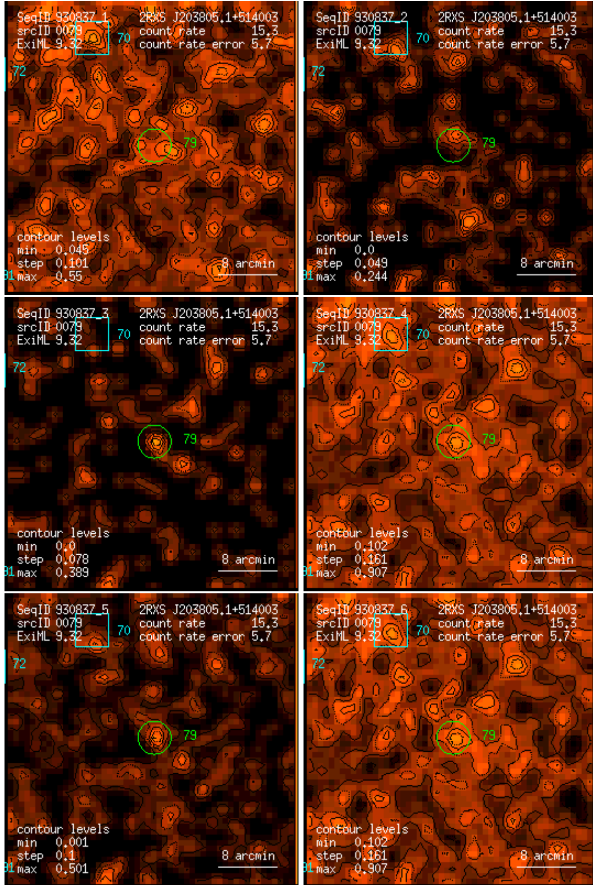
Figure 79: RASS 930837: detection 0079: band rate images, Gaussian filter: (1) PSPC channels 11 – 41, (2) 52 – 90, (3) 91 – 201, (4) 11 – 235, (5) 52 – 201, (6) 11 – 201. Broad band rates in counts/ks. Band rate contour levels in counts/ks/arcmin 2 .
