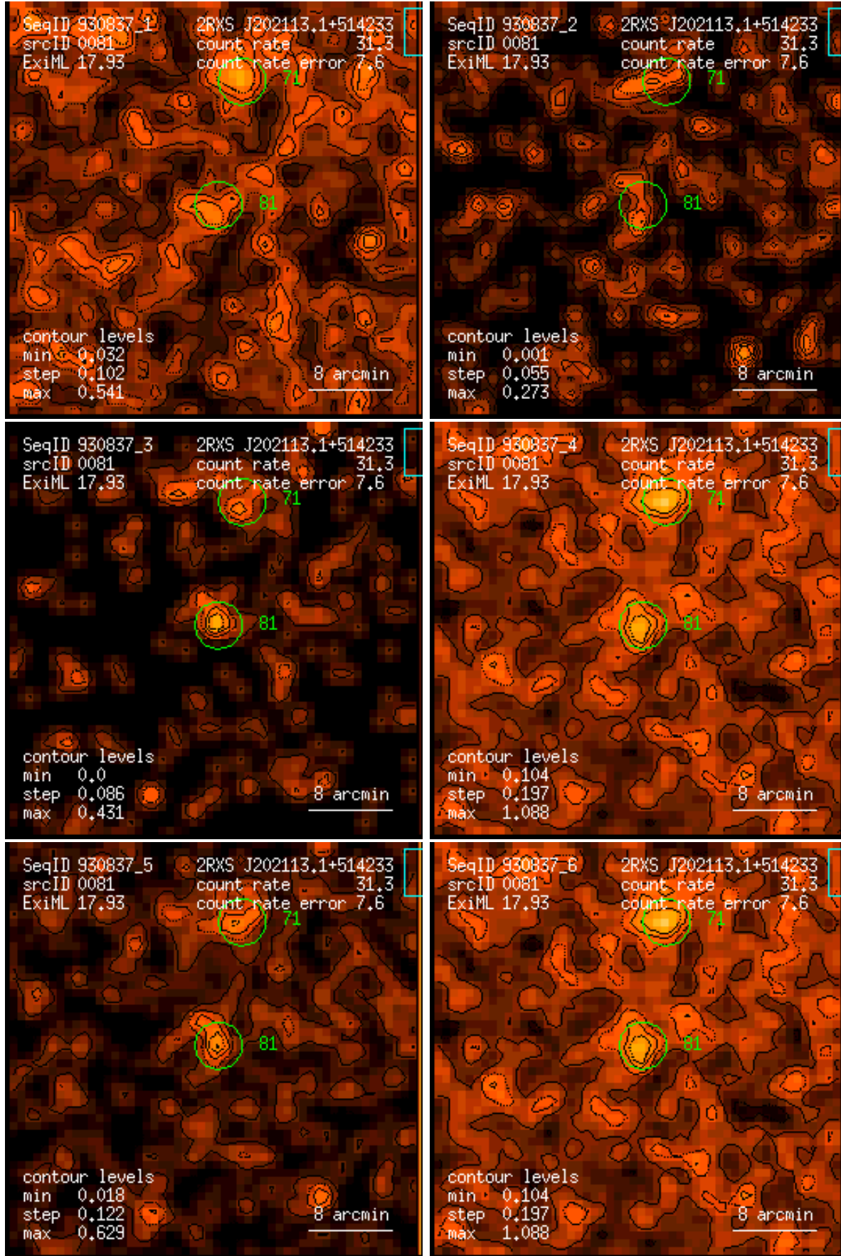
Figure 81: RASS 930837: detection 0081: band rate images, Gaussian filter: (1) PSPC channels 11 – 41, (2) 52 – 90, (3) 91 – 201, (4) 11 – 235, (5) 52 – 201, (6) 11 – 201. Broad band rates in counts/ks. Band rate contour levels in counts/ks/arcmin 2 .
