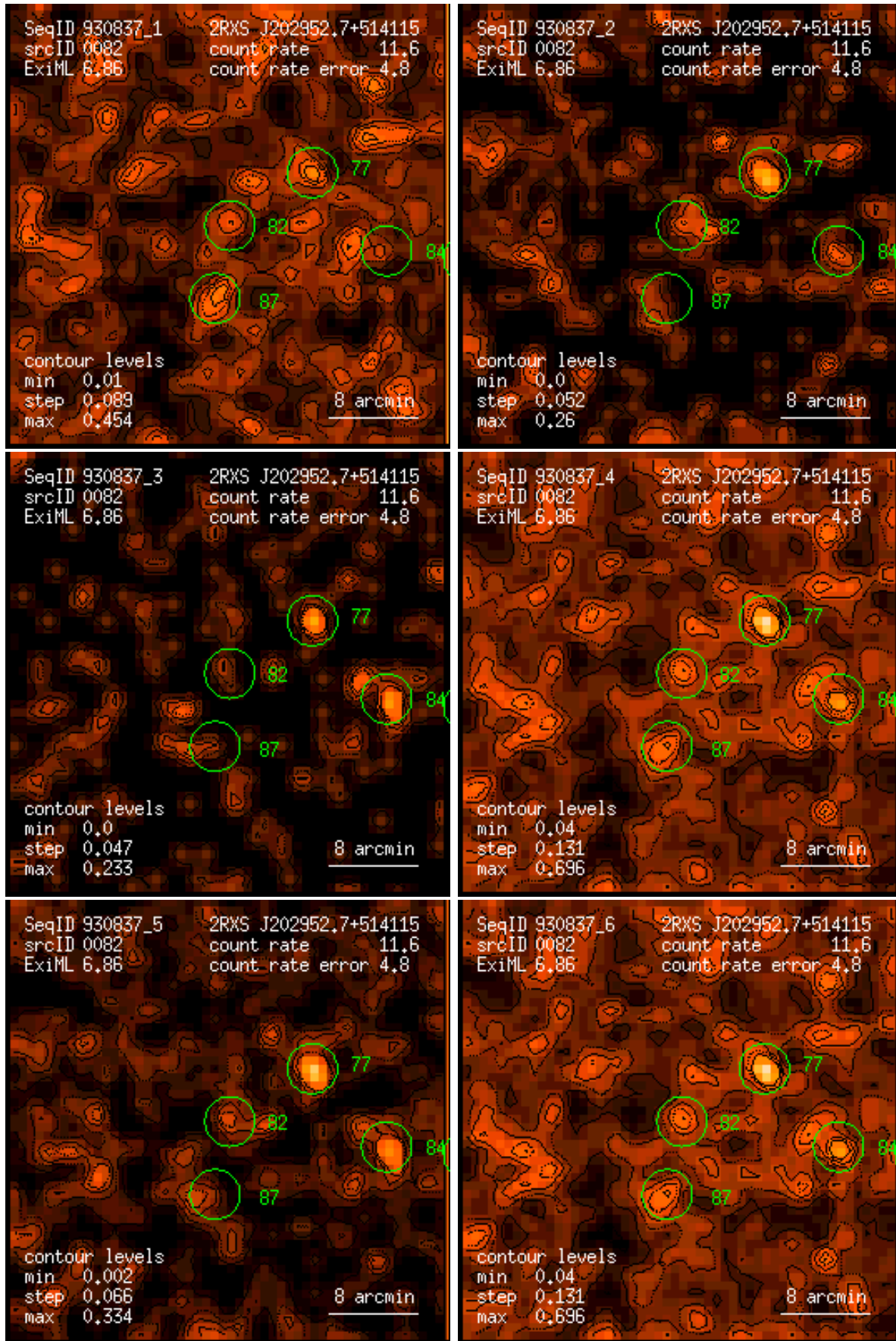
Figure 82: RASS 930837: detection 0082: band rate images, Gaussian filter: (1) PSPC channels 11 – 41, (2) 52 – 90, (3) 91 – 201, (4) 11 – 235, (5) 52 – 201, (6) 11 – 201. Broad band rates in counts/ks. Band rate contour levels in counts/ks/arcmin 2 .
