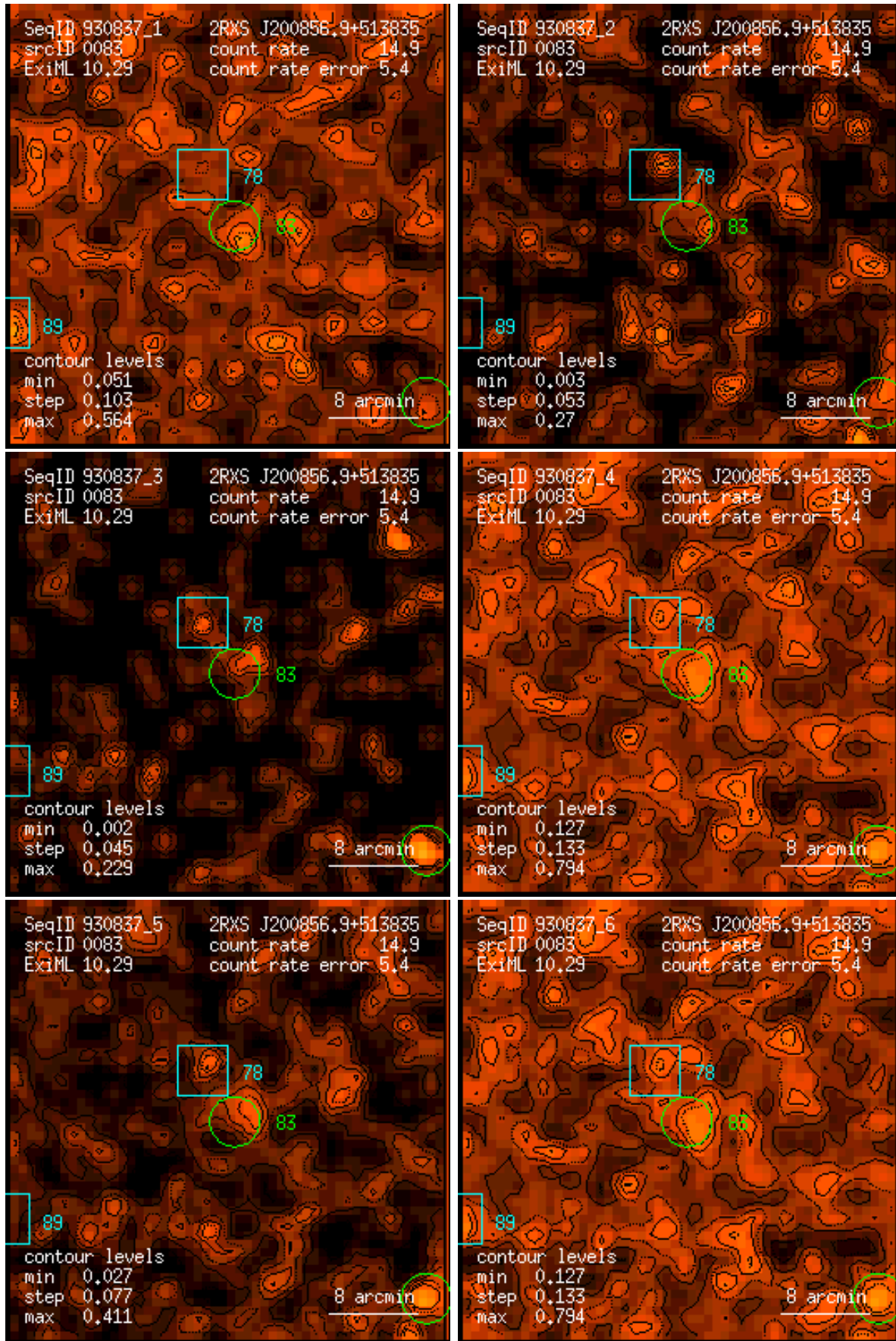
Figure 83: RASS 930837: detection 0083: band rate images, Gaussian filter: (1) PSPC channels 11 – 41, (2) 52 – 90, (3) 91 – 201, (4) 11 – 235, (5) 52 – 201, (6) 11 – 201. Broad band rates in counts/ks. Band rate contour levels in counts/ks/arcmin 2 .
