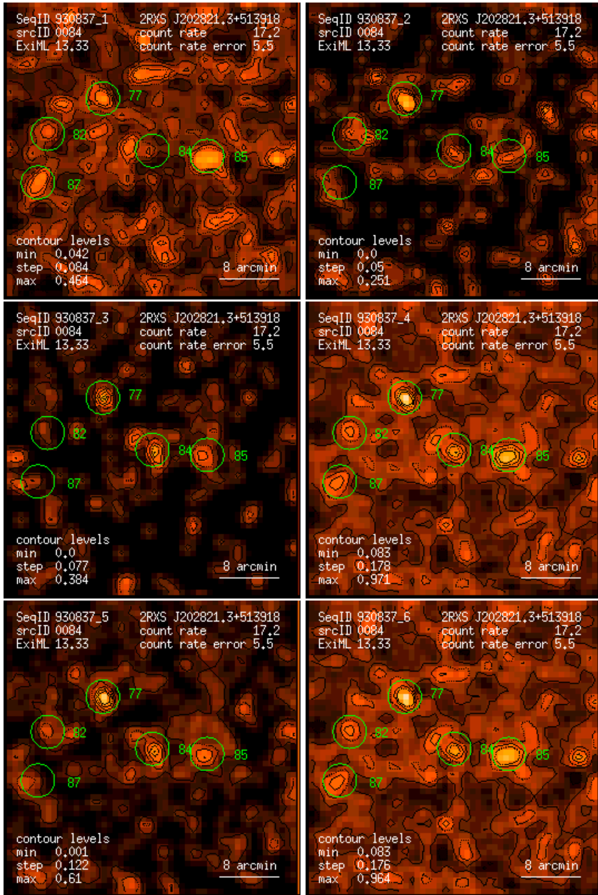
Figure 84: RASS 930837: detection 0084: band rate images, Gaussian filter: (1) PSPC channels 11 – 41, (2) 52 – 90, (3) 91 – 201, (4) 11 – 235, (5) 52 – 201, (6) 11 – 201. Broad band rates in counts/ks. Band rate contour levels in counts/ks/arcmin 2 .
