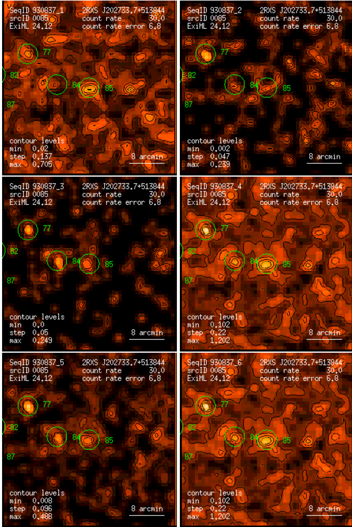
Figure 85: RASS 930837: detection 0085: band rate images, Gaussian filter: (1) PSPC channels 11 – 41, (2) 52 – 90, (3) 91 – 201, (4) 11 – 235, (5) 52 – 201, (6) 11 – 201. Broad band rates in counts/ks. Band rate contour levels in counts/ks/arcmin 2 .
