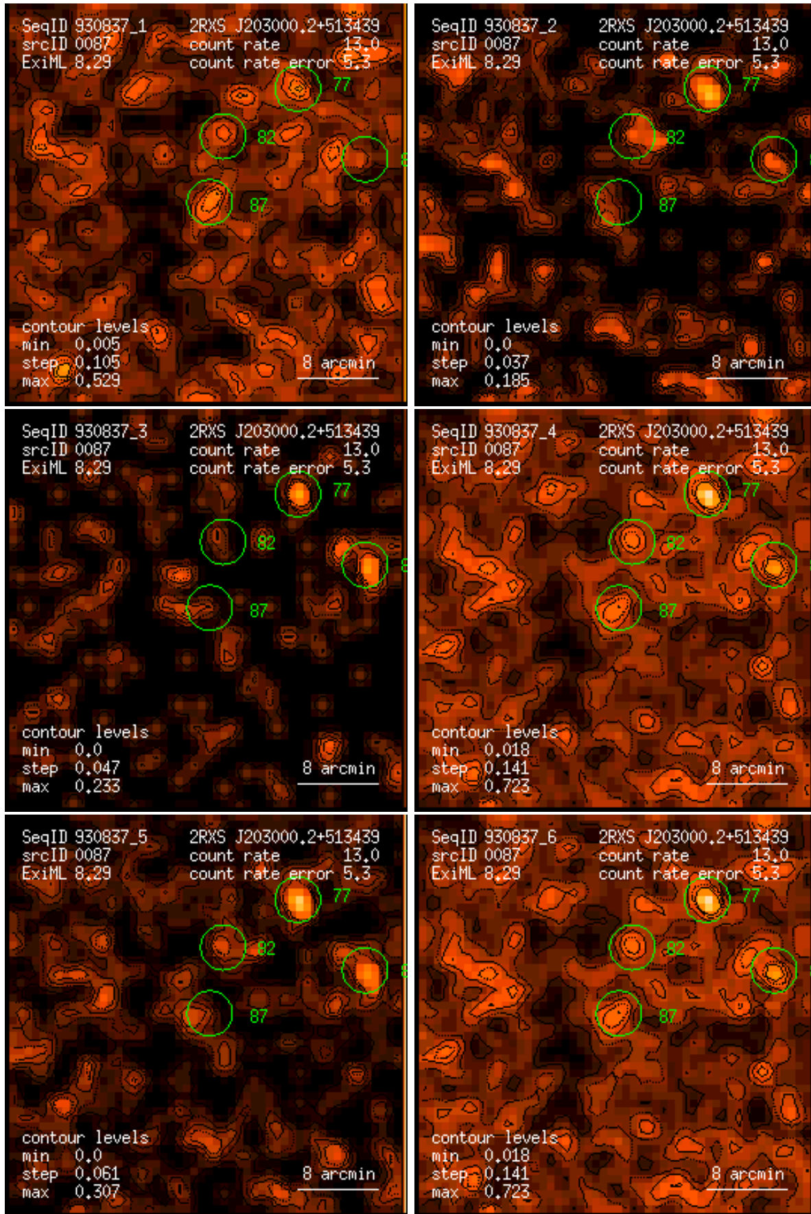
Figure 87: RASS 930837: detection 0087: band rate images, Gaussian filter: (1) PSPC channels 11 – 41, (2) 52 – 90, (3) 91 – 201, (4) 11 – 235, (5) 52 – 201, (6) 11 – 201. Broad band rates in counts/ks. Band rate contour levels in counts/ks/arcmin 2 .
