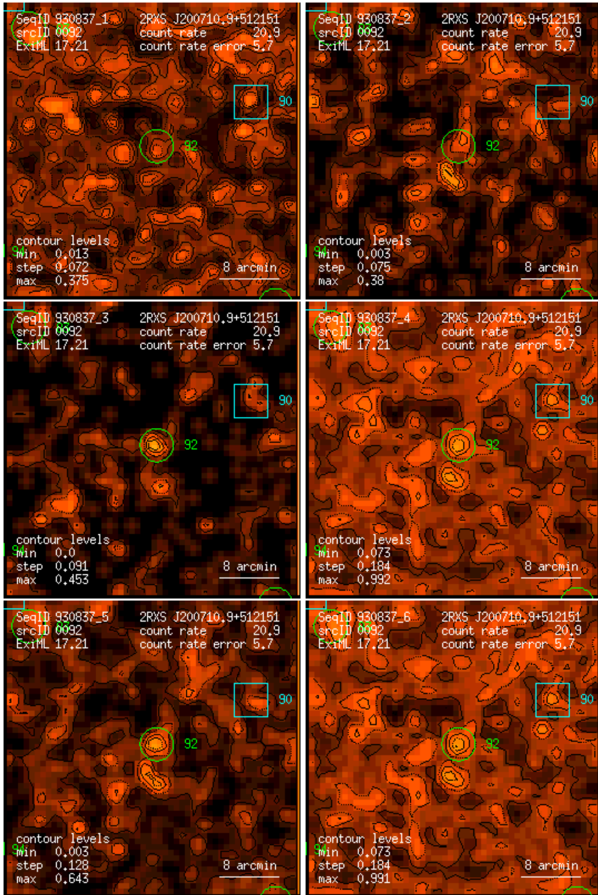
Figure 92: RASS 930837: detection 0092: band rate images, Gaussian filter: (1) PSPC channels 11 – 41, (2) 52 – 90, (3) 91 – 201, (4) 11 – 235, (5) 52 – 201, (6) 11 – 201. Broad band rates in counts/ks. Band rate contour levels in counts/ks/arcmin 2 .
