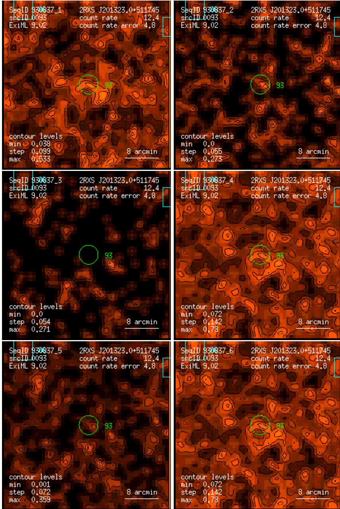
Figure 93: RASS 930837: detection 0093: band rate images, Gaussian filter: (1) PSPC channels 11 – 41, (2) 52 – 90, (3) 91 – 201, (4) 11 – 235, (5) 52 – 201, (6) 11 – 201. Broad band rates in counts/ks. Band rate contour levels in counts/ks/arcmin 2 .
