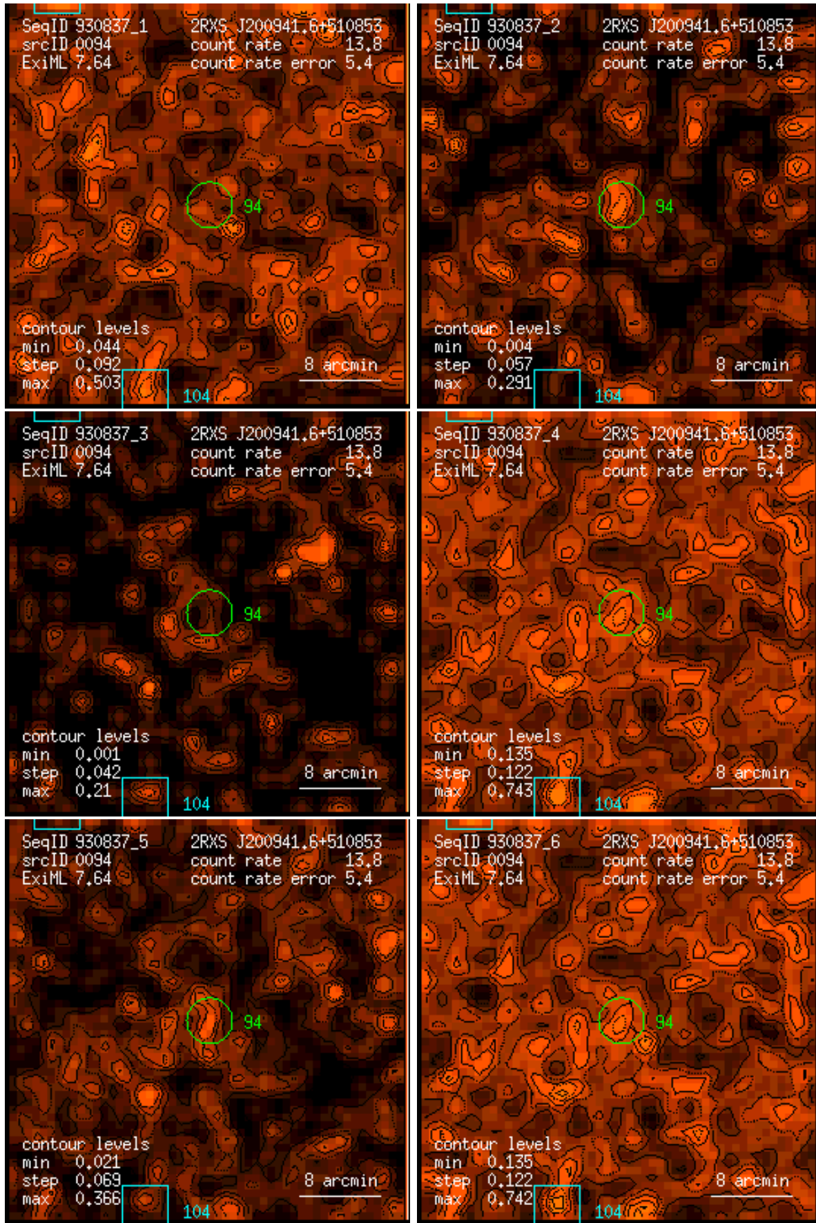
Figure 94: RASS 930837: detection 0094: band rate images, Gaussian filter: (1) PSPC channels 11 – 41, (2) 52 – 90, (3) 91 – 201, (4) 11 – 235, (5) 52 – 201, (6) 11 – 201. Broad band rates in counts/ks. Band rate contour levels in counts/ks/arcmin 2 .
