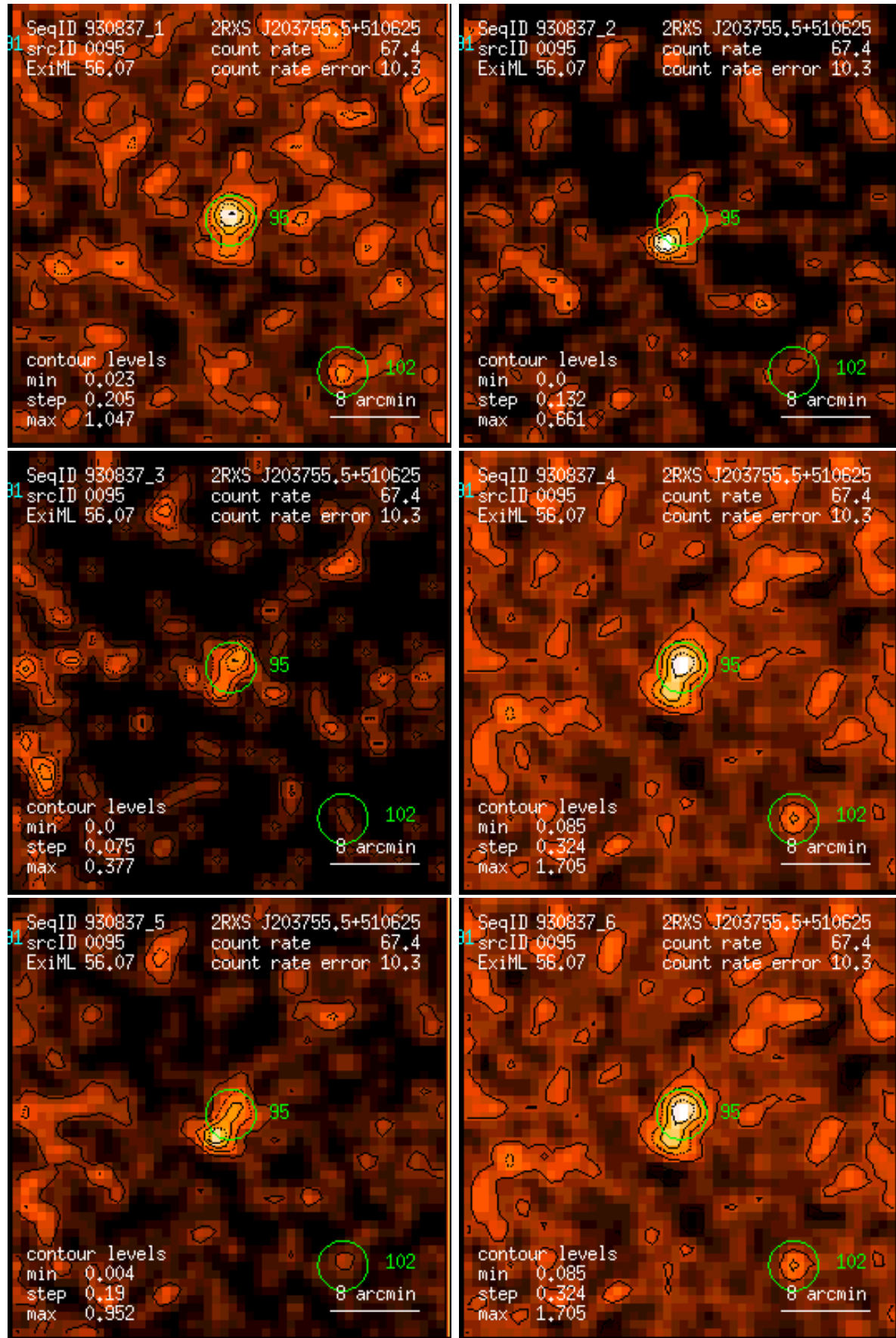
Figure 95: RASS 930837: detection 0095: band rate images, Gaussian filter: (1) PSPC channels 11 – 41, (2) 52 – 90, (3) 91 – 201, (4) 11 – 235, (5) 52 – 201, (6) 11 – 201. Broad band rates in counts/ks. Band rate contour levels in counts/ks/arcmin 2 .
