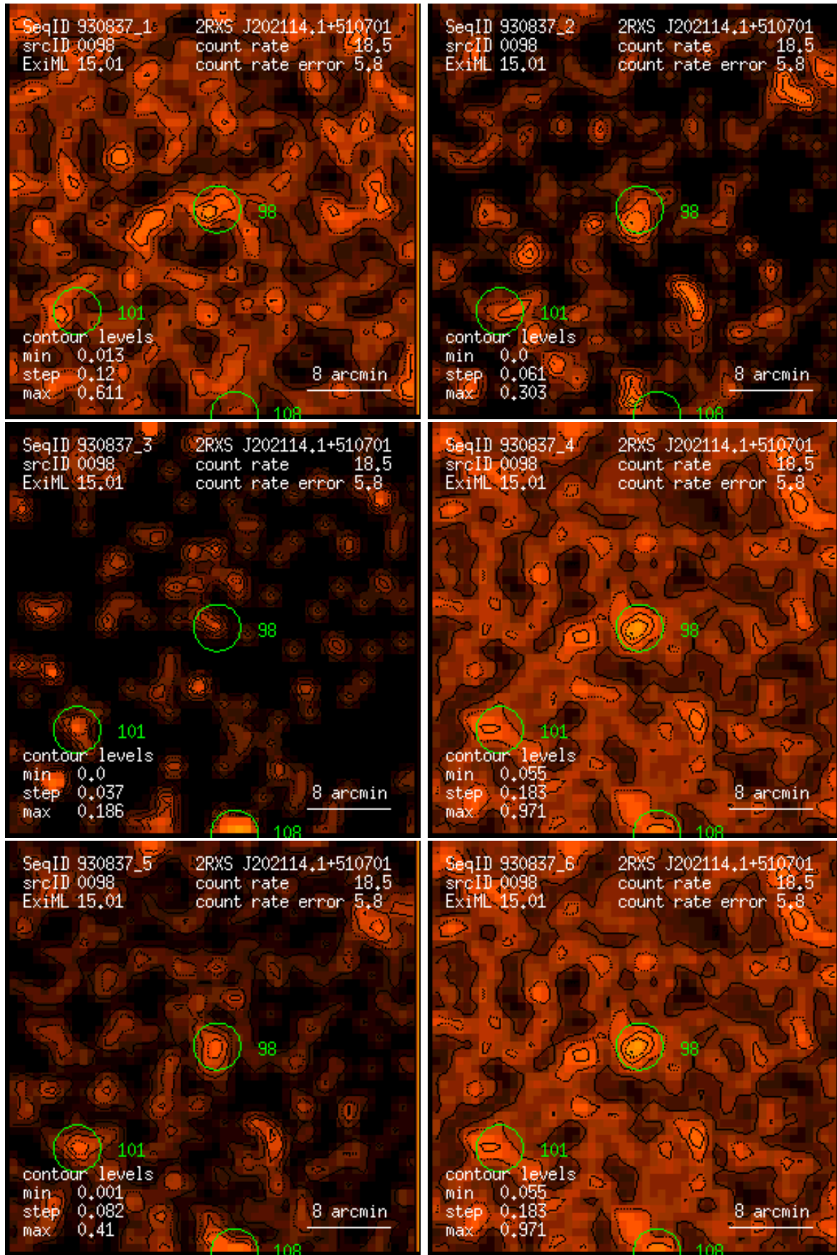
Figure 98: RASS 930837: detection 0098: band rate images, Gaussian filter: (1) PSPC channels 11 – 41, (2) 52 – 90, (3) 91 – 201, (4) 11 – 235, (5) 52 – 201, (6) 11 – 201. Broad band rates in counts/ks. Band rate contour levels in counts/ks/arcmin 2 .
