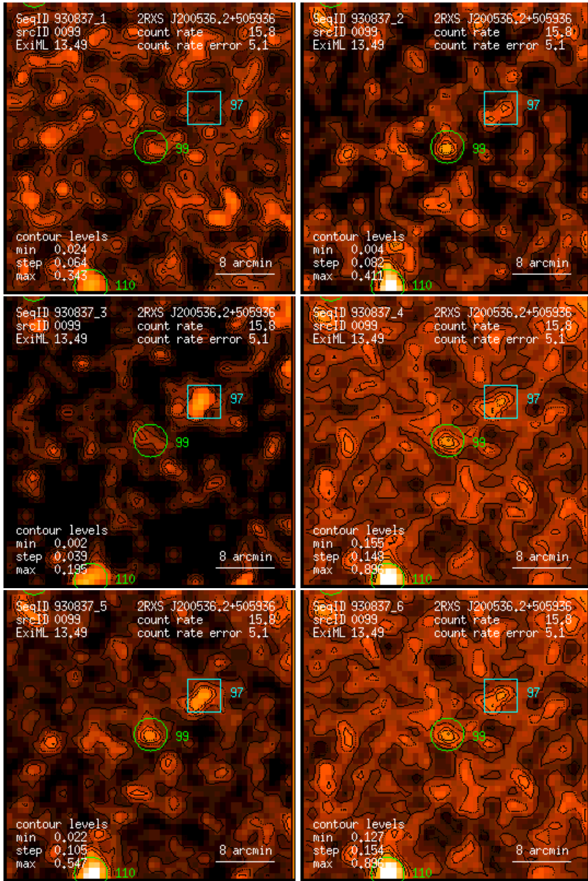
Figure 99: RASS 930837: detection 0099: band rate images, Gaussian filter: (1) PSPC channels 11 – 41, (2) 52 – 90, (3) 91 – 201, (4) 11 – 235, (5) 52 – 201, (6) 11 – 201. Broad band rates in counts/ks. Band rate contour levels in counts/ks/arcmin 2 .
