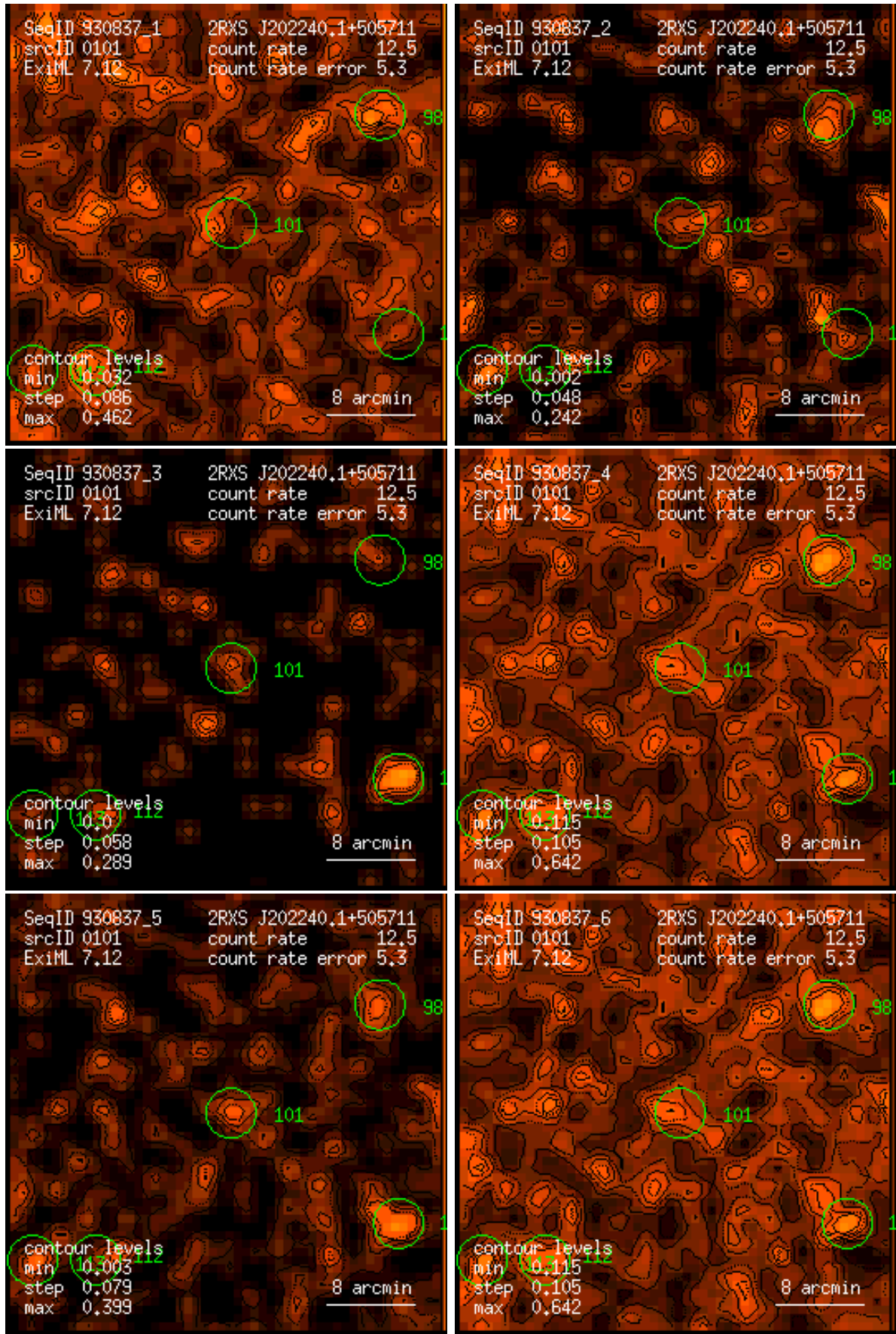
Figure 101: RASS 930837: detection 0101: band rate images, Gaussian filter: (1) PSPC channels 11 – 41, (2) 52 – 90, (3) 91 – 201, (4) 11 – 235, (5) 52 – 201, (6) 11 – 201. Broad band rates in counts/ks. Band rate contour levels in counts/ks/arcmin 2 .
