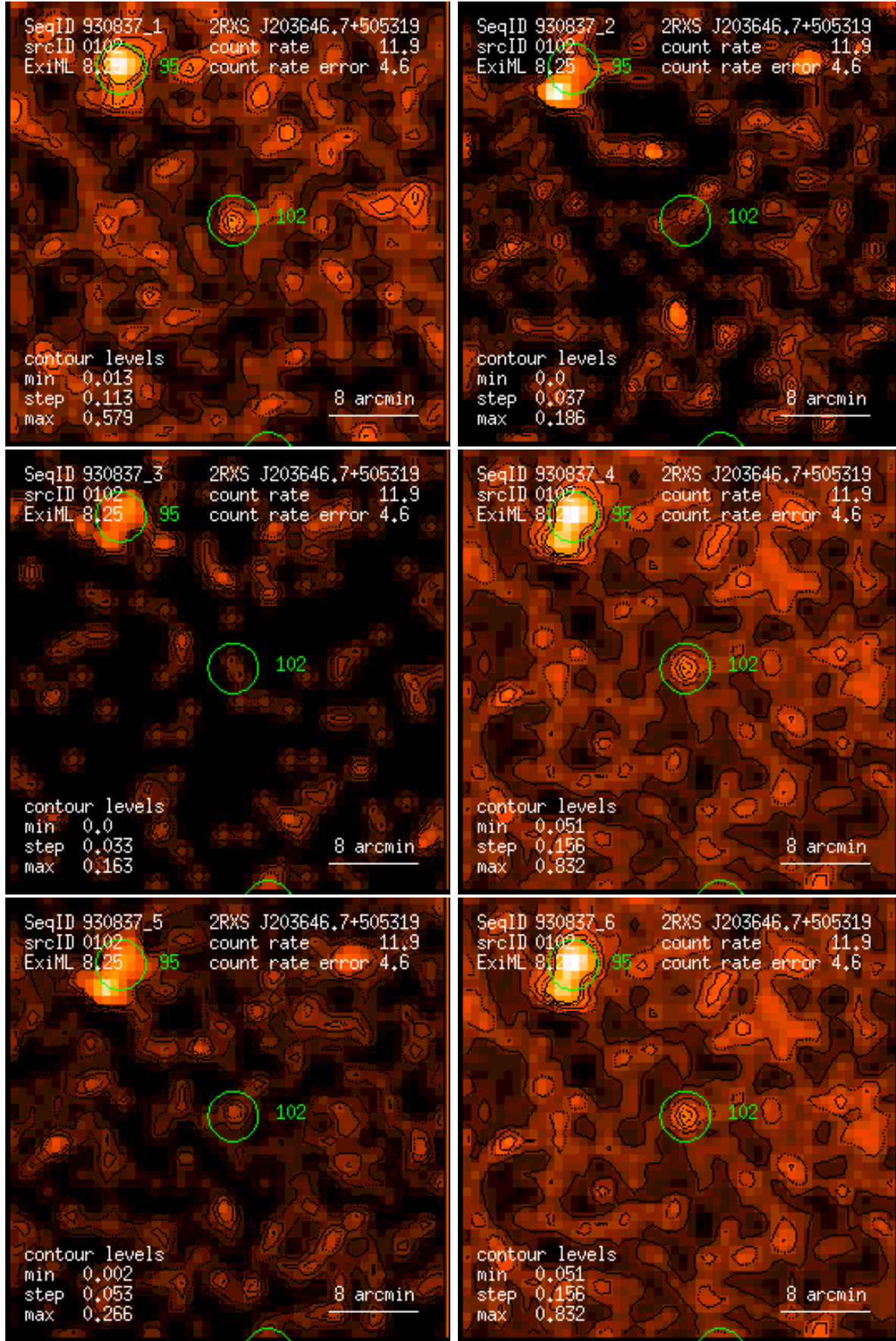
Figure 102: RASS 930837: detection 0102: band rate images, Gaussian filter: (1) PSPC channels 11 – 41, (2) 52 – 90, (3) 91 – 201, (4) 11 – 235, (5) 52 – 201, (6) 11 – 201. Broad band rates in counts/ks. Band rate contour levels in counts/ks/arcmin 2 .
