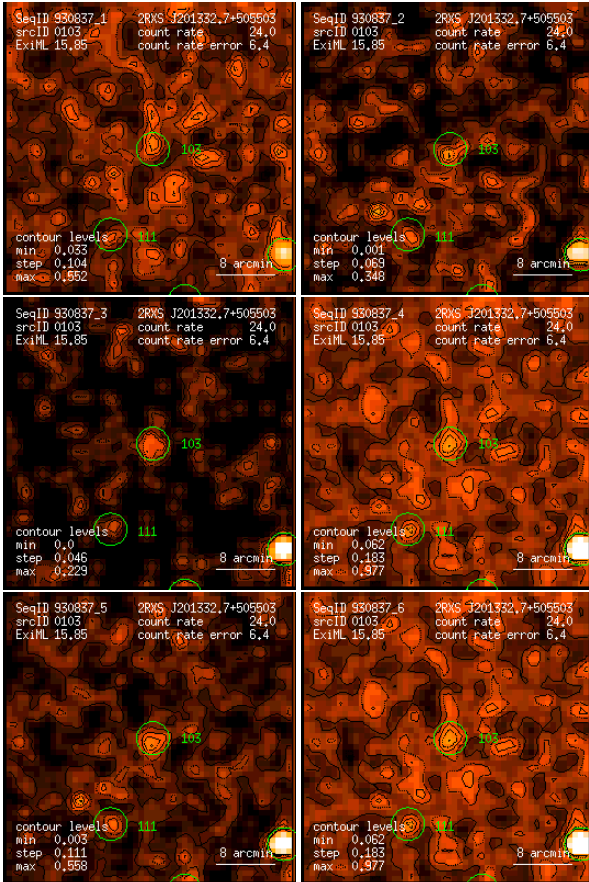
Figure 103: RASS 930837: detection 0103: band rate images, Gaussian filter: (1) PSPC channels 11 – 41, (2) 52 – 90, (3) 91 – 201, (4) 11 – 235, (5) 52 – 201, (6) 11 – 201. Broad band rates in counts/ks. Band rate contour levels in counts/ks/arcmin 2 .
