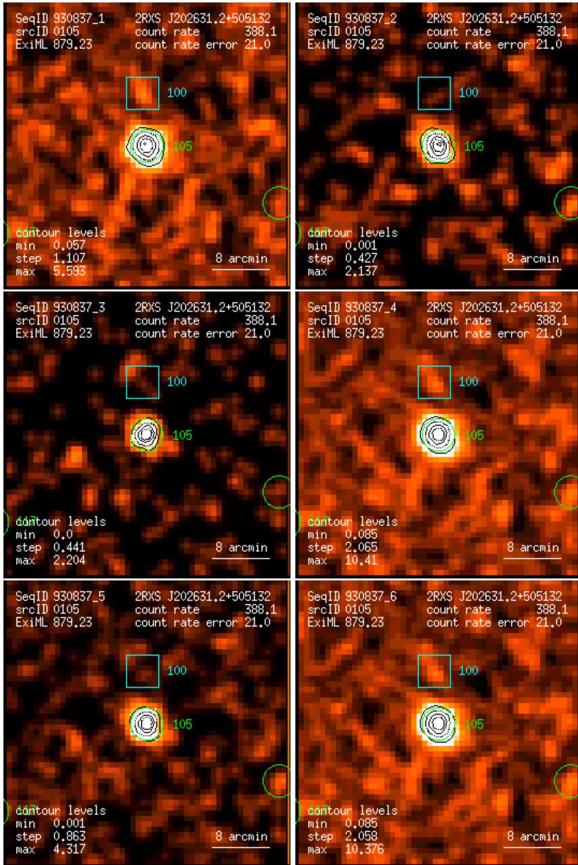
Figure 105: RASS 930837: detection 0105: band rate images, Gaussian filter: (1) PSPC channels 11 – 41, (2) 52 – 90, (3) 91 – 201, (4) 11 – 235, (5) 52 – 201, (6) 11 – 201. Broad band rates in counts/ks. Band rate contour levels in counts/ks/arcmin 2 .
