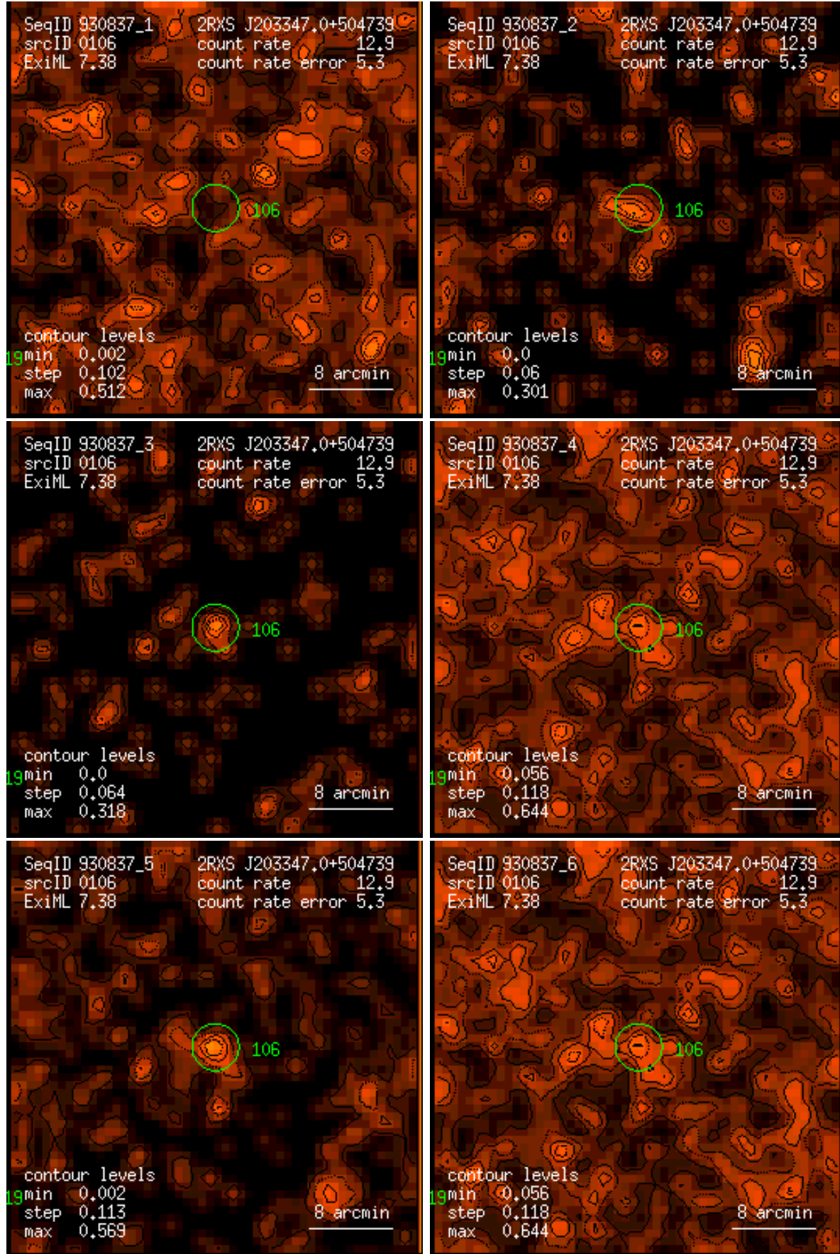
Figure 106: RASS 930837: detection 0106: band rate images, Gaussian filter: (1) PSPC channels 11 – 41, (2) 52 – 90, (3) 91 – 201, (4) 11 – 235, (5) 52 – 201, (6) 11 – 201. Broad band rates in counts/ks. Band rate contour levels in counts/ks/arcmin 2 .
