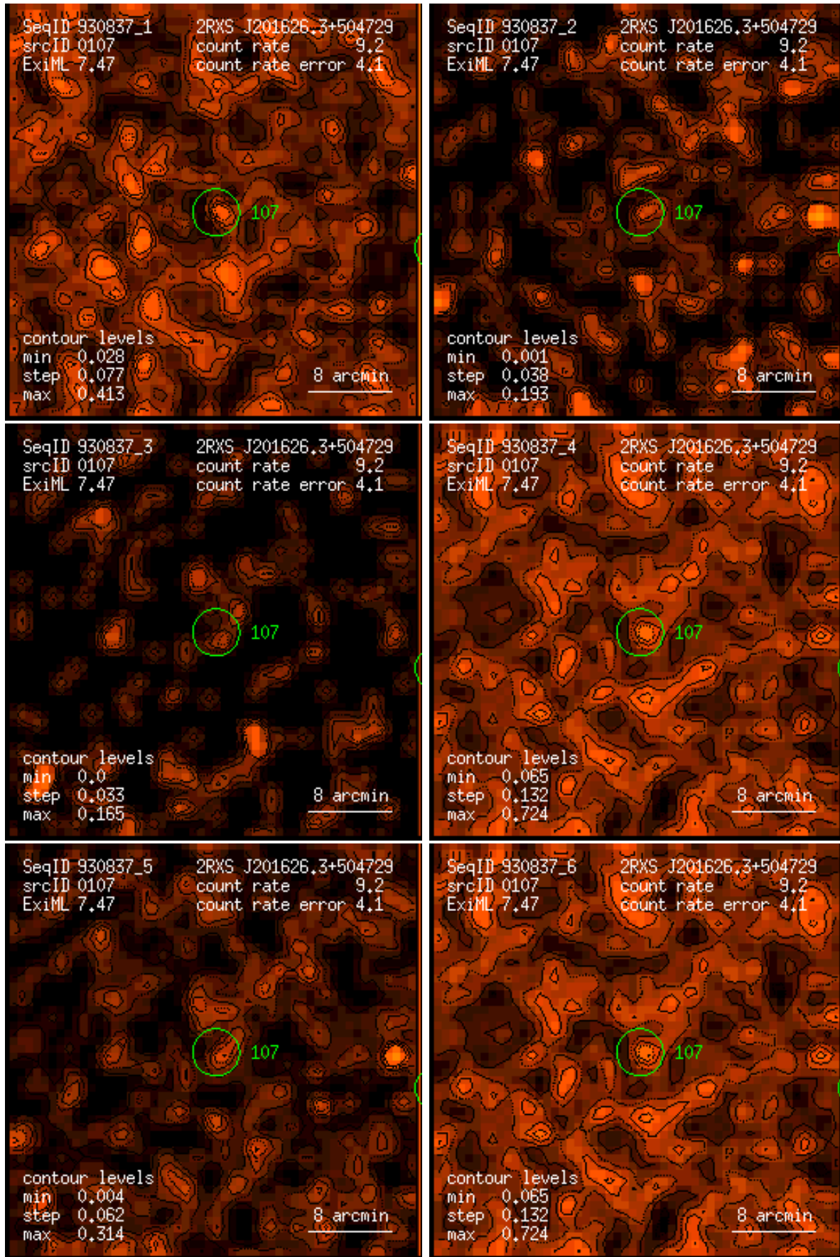
Figure 107: RASS 930837: detection 0107: band rate images, Gaussian filter: (1) PSPC channels 11 – 41, (2) 52 – 90, (3) 91 – 201, (4) 11 – 235, (5) 52 – 201, (6) 11 – 201. Broad band rates in counts/ks. Band rate contour levels in counts/ks/arcmin 2 .
