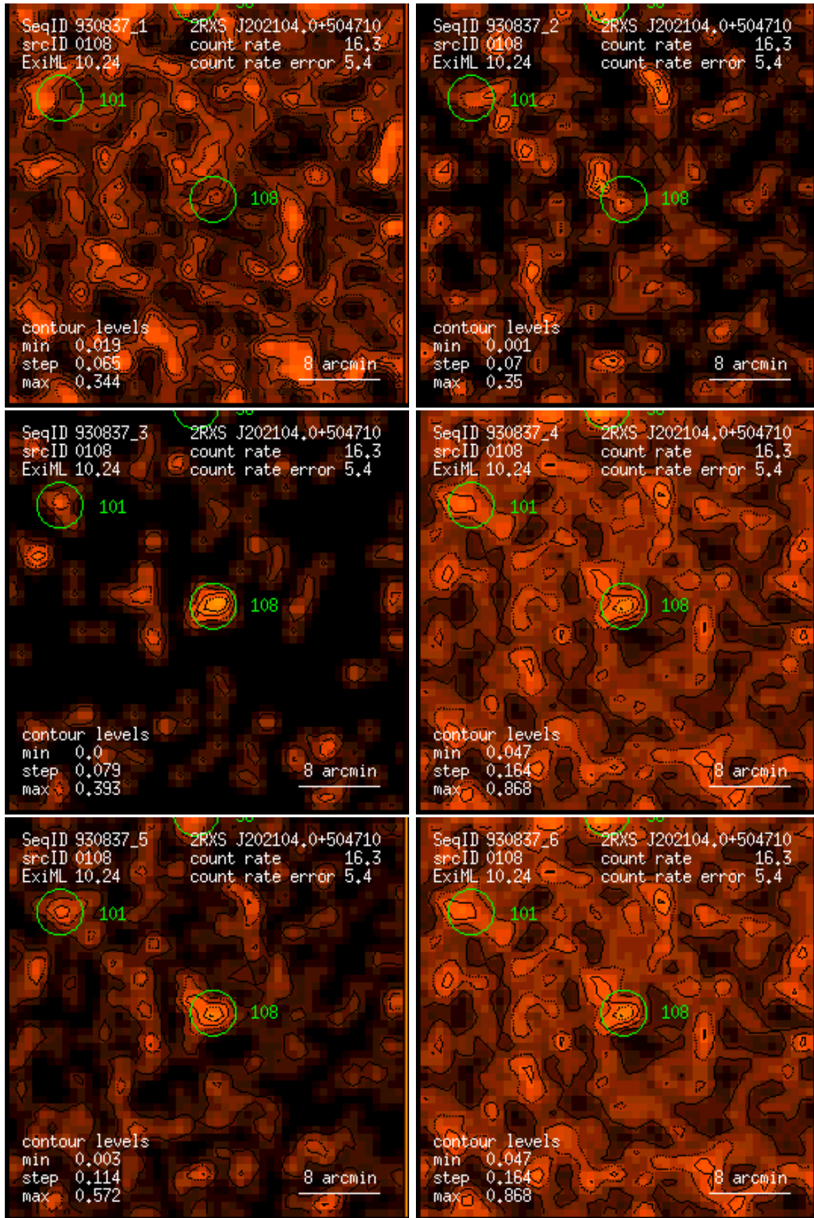
Figure 108: RASS 930837: detection 0108: band rate images, Gaussian filter: (1) PSPC channels 11 – 41, (2) 52 – 90, (3) 91 – 201, (4) 11 – 235, (5) 52 – 201, (6) 11 – 201. Broad band rates in counts/ks. Band rate contour levels in counts/ks/arcmin 2 .
