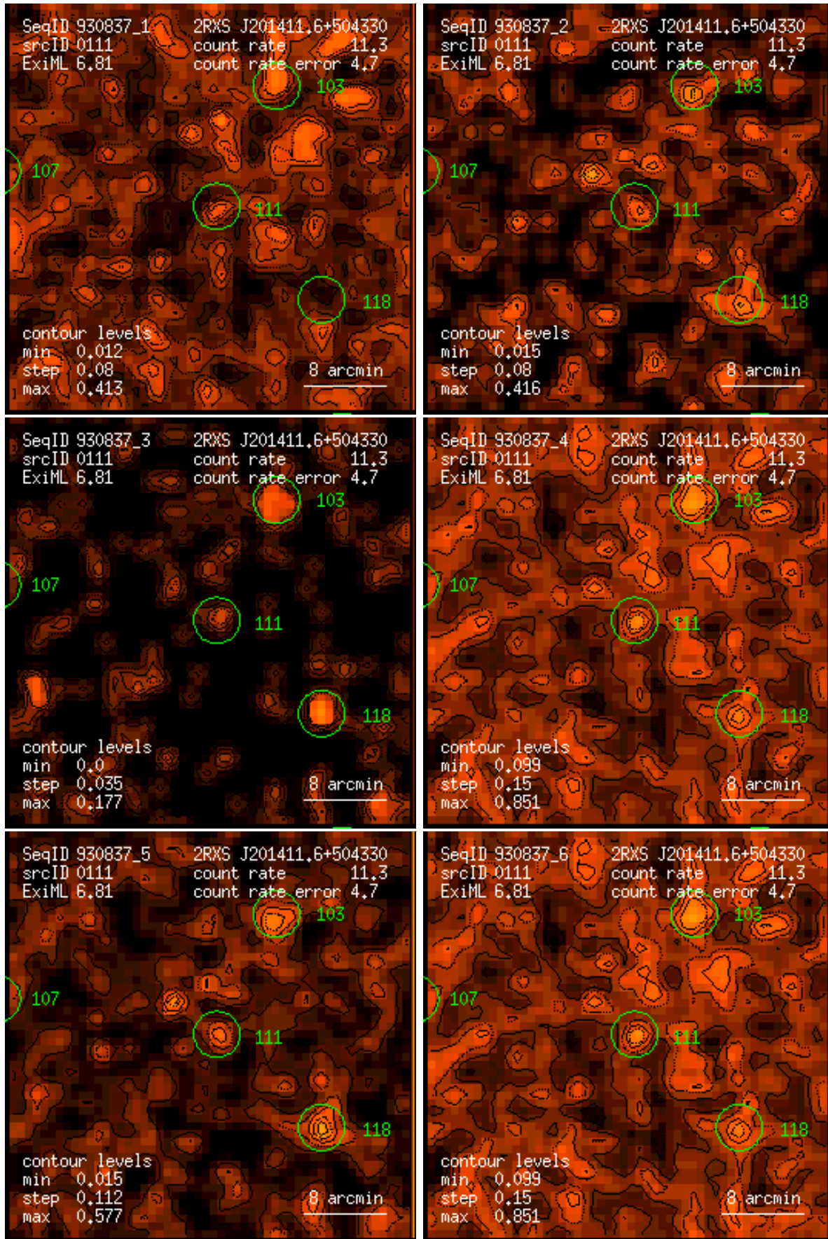
Figure 111: RASS 930837: detection 0111: band rate images, Gaussian filter: (1) PSPC channels 11 – 41, (2) 52 – 90, (3) 91 – 201, (4) 11 – 235, (5) 52 – 201, (6) 11 – 201. Broad band rates in counts/ks. Band rate contour levels in counts/ks/arcmin 2 .
