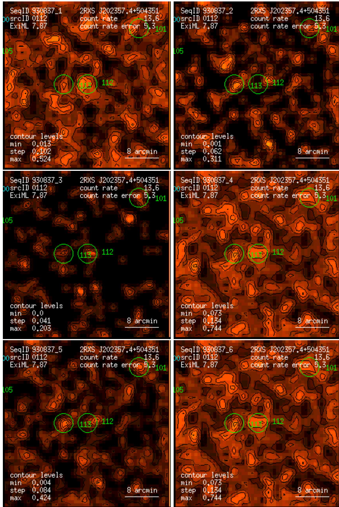
Figure 112: RASS 930837: detection 0112: band rate images, Gaussian filter: (1) PSPC channels 11 – 41, (2) 52 – 90, (3) 91 – 201, (4) 11 – 235, (5) 52 – 201, (6) 11 – 201. Broad band rates in counts/ks. Band rate contour levels in counts/ks/arcmin 2 .
