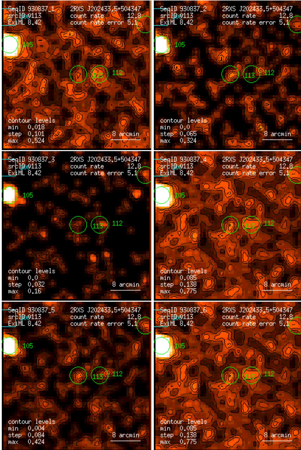
Figure 113: RASS 930837: detection 0113: band rate images, Gaussian filter: (1) PSPC channels 11 – 41, (2) 52 – 90, (3) 91 – 201, (4) 11 – 235, (5) 52 – 201, (6) 11 – 201. Broad band rates in counts/ks. Band rate contour levels in counts/ks/arcmin 2 .
