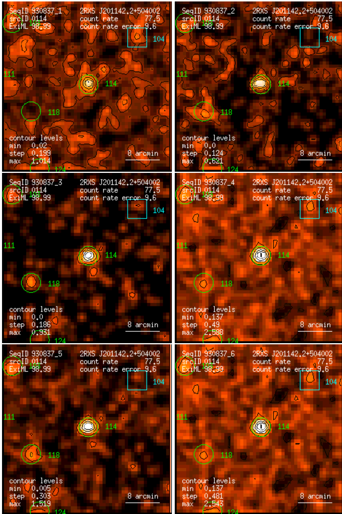
Figure 114: RASS 930837: detection 0114: band rate images, Gaussian filter: (1) PSPC channels 11 – 41, (2) 52 – 90, (3) 91 – 201, (4) 11 – 235, (5) 52 – 201, (6) 11 – 201. Broad band rates in counts/ks. Band rate contour levels in counts/ks/arcmin 2 .
