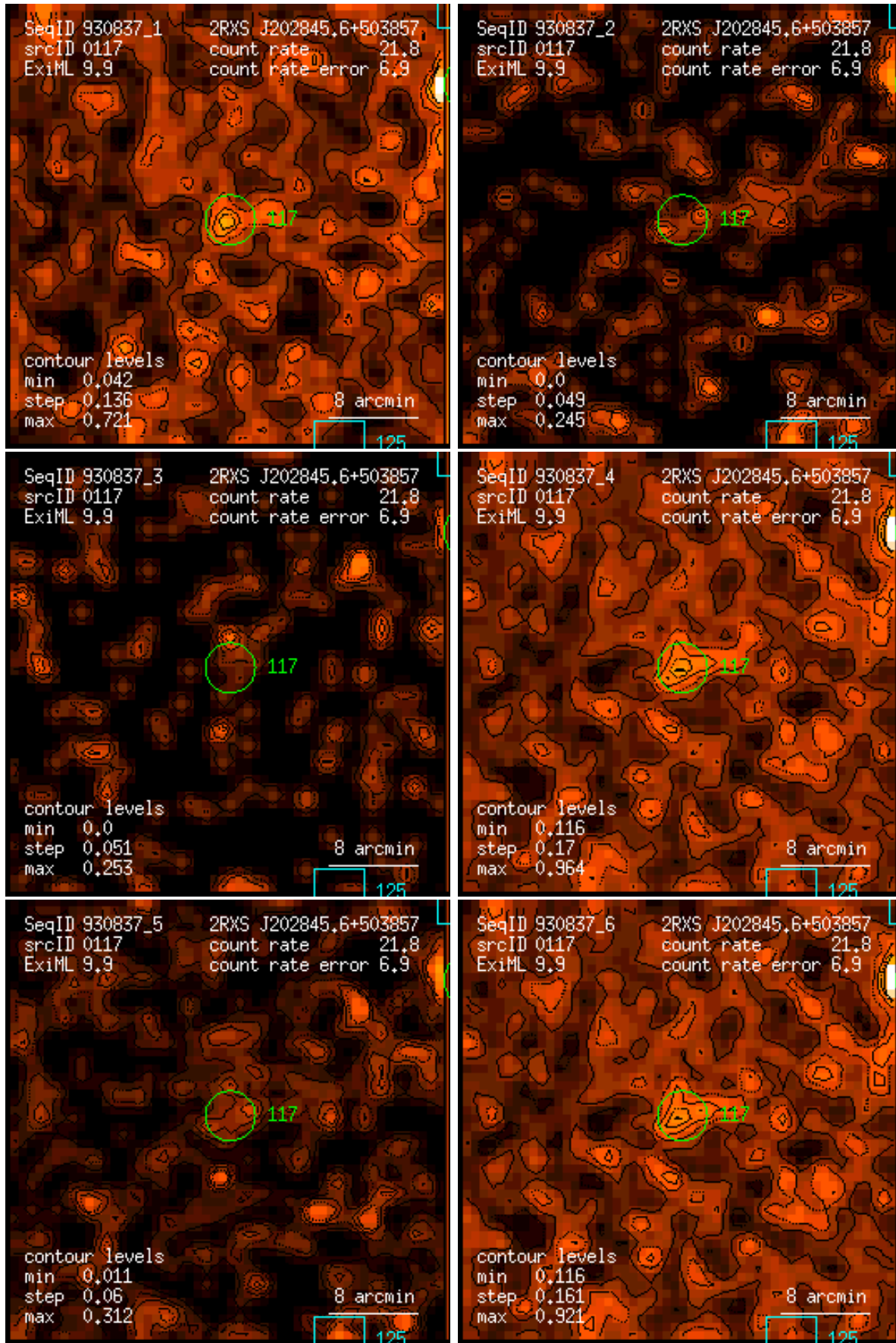
Figure 117: RASS 930837: detection 0117: band rate images, Gaussian filter: (1) PSPC channels 11 – 41, (2) 52 – 90, (3) 91 – 201, (4) 11 – 235, (5) 52 – 201, (6) 11 – 201. Broad band rates in counts/ks. Band rate contour levels in counts/ks/arcmin 2 .
