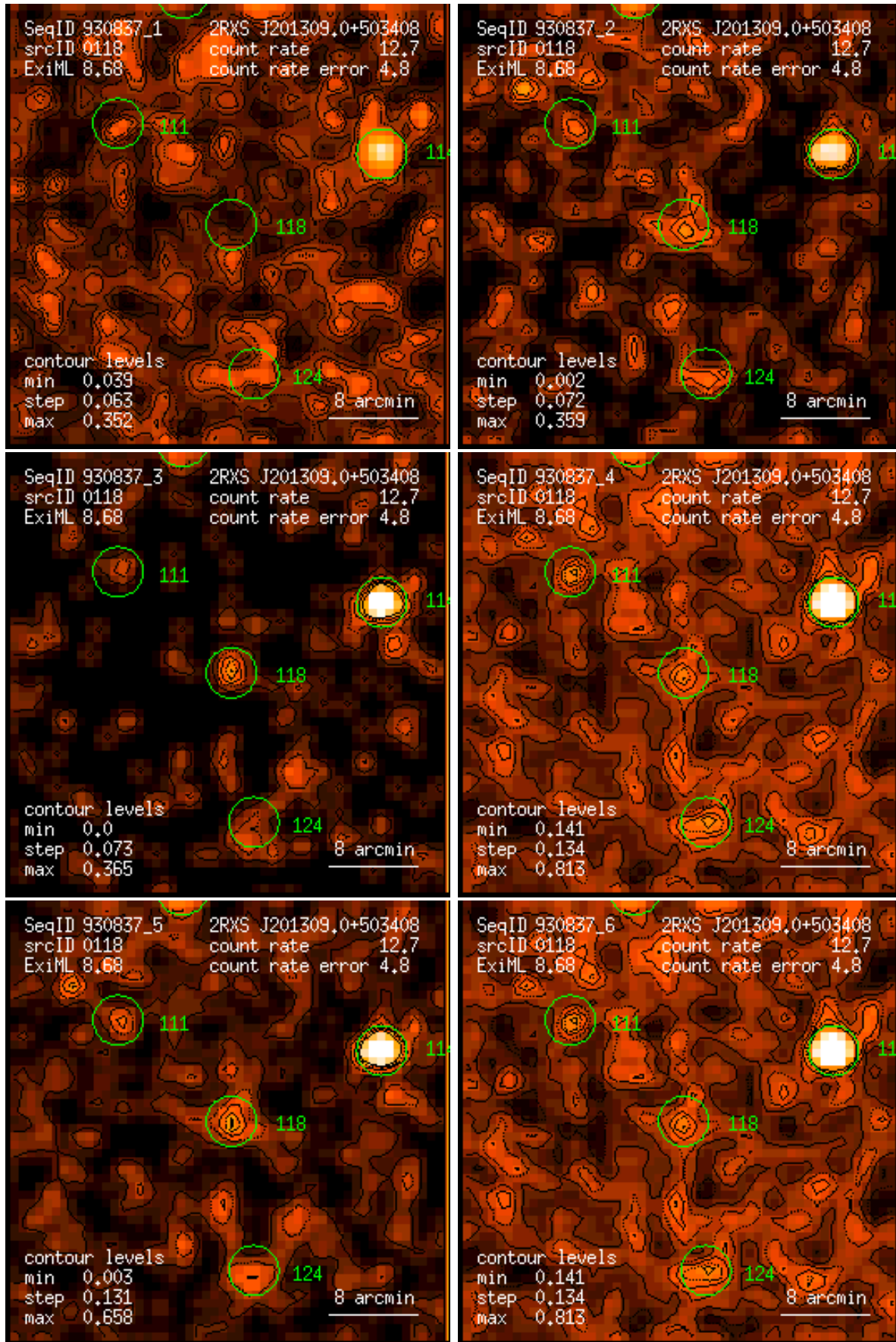
Figure 118: RASS 930837: detection 0118: band rate images, Gaussian filter: (1) PSPC channels 11 – 41, (2) 52 – 90, (3) 91 – 201, (4) 11 – 235, (5) 52 – 201, (6) 11 – 201. Broad band rates in counts/ks. Band rate contour levels in counts/ks/arcmin 2 .
