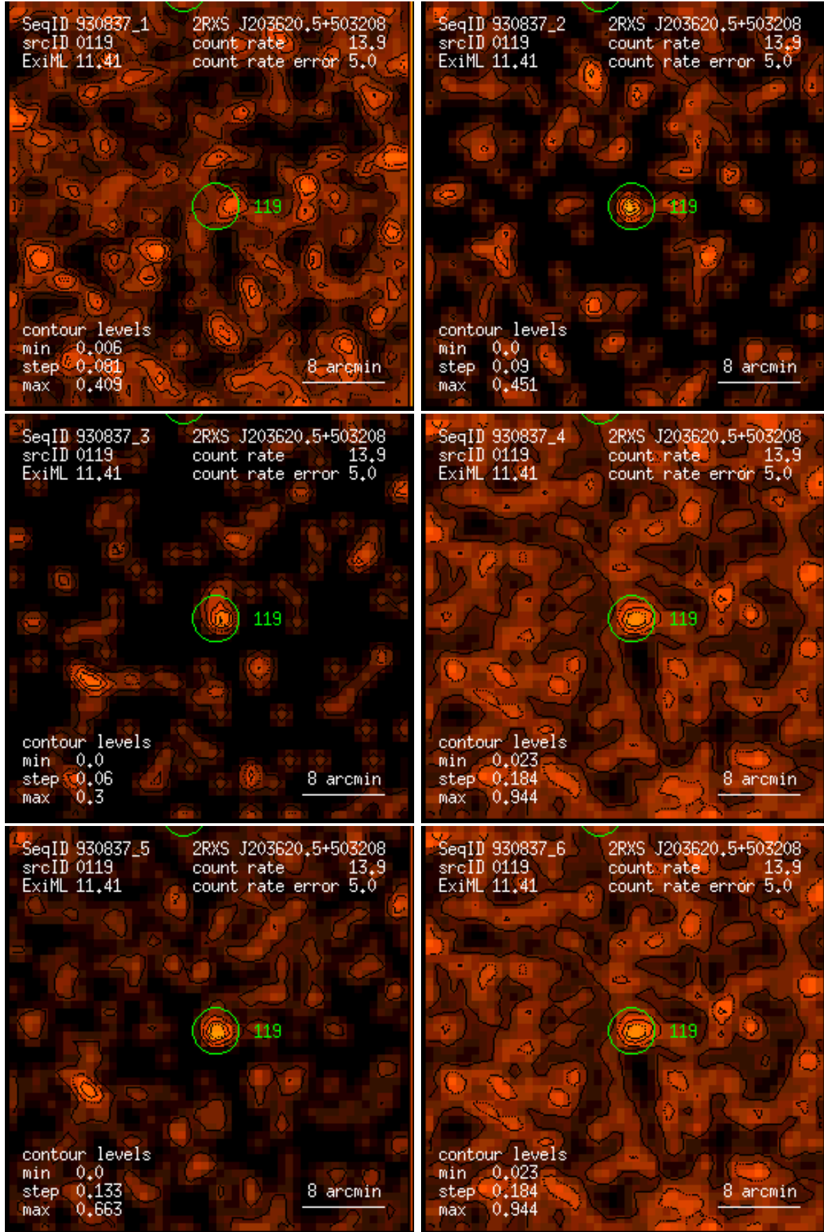
Figure 119: RASS 930837: detection 0119: band rate images, Gaussian filter: (1) PSPC channels 11 – 41, (2) 52 – 90, (3) 91 – 201, (4) 11 – 235, (5) 52 – 201, (6) 11 – 201. Broad band rates in counts/ks. Band rate contour levels in counts/ks/arcmin 2 .
