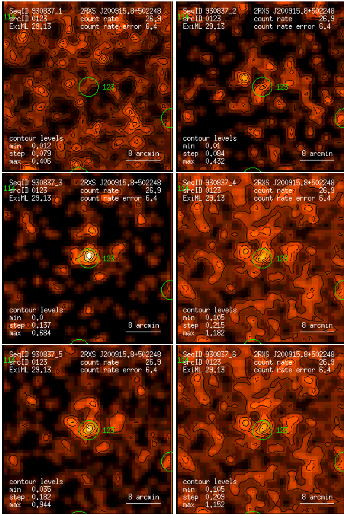
Figure 123: RASS 930837: detection 0123: band rate images, Gaussian filter: (1) PSPC channels 11 – 41, (2) 52 – 90, (3) 91 – 201, (4) 11 – 235, (5) 52 – 201, (6) 11 – 201. Broad band rates in counts/ks. Band rate contour levels in counts/ks/arcmin 2 .
