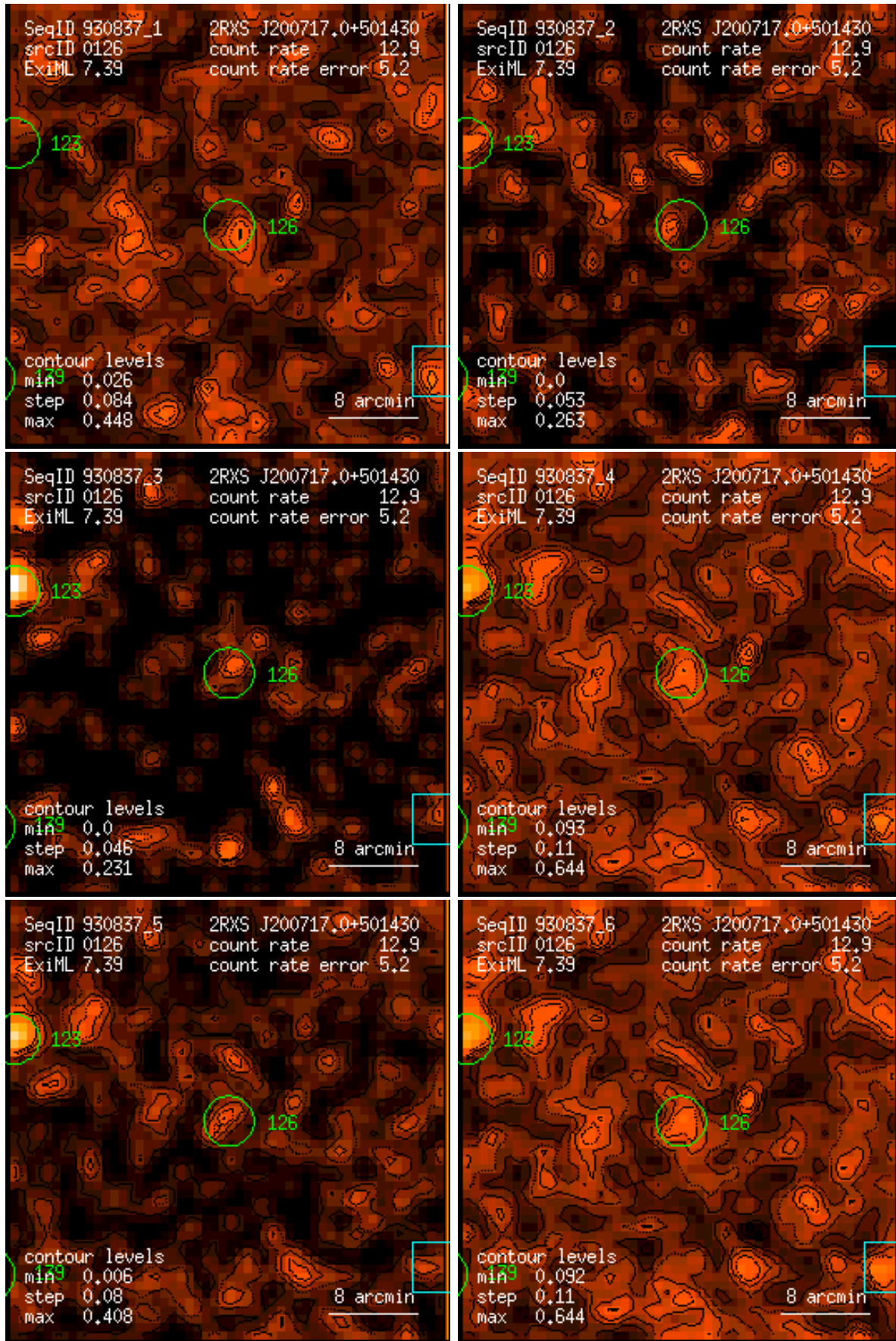
Figure 126: RASS 930837: detection 0126: band rate images, Gaussian filter: (1) PSPC channels 11 – 41, (2) 52 – 90, (3) 91 – 201, (4) 11 – 235, (5) 52 – 201, (6) 11 – 201. Broad band rates in counts/ks. Band rate contour levels in counts/ks/arcmin 2 .
