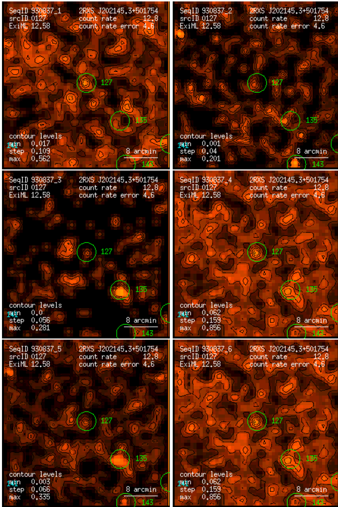
Figure 127: RASS 930837: detection 0127: band rate images, Gaussian filter: (1) PSPC channels 11 – 41, (2) 52 – 90, (3) 91 – 201, (4) 11 – 235, (5) 52 – 201, (6) 11 – 201. Broad band rates in counts/ks. Band rate contour levels in counts/ks/arcmin 2 .
