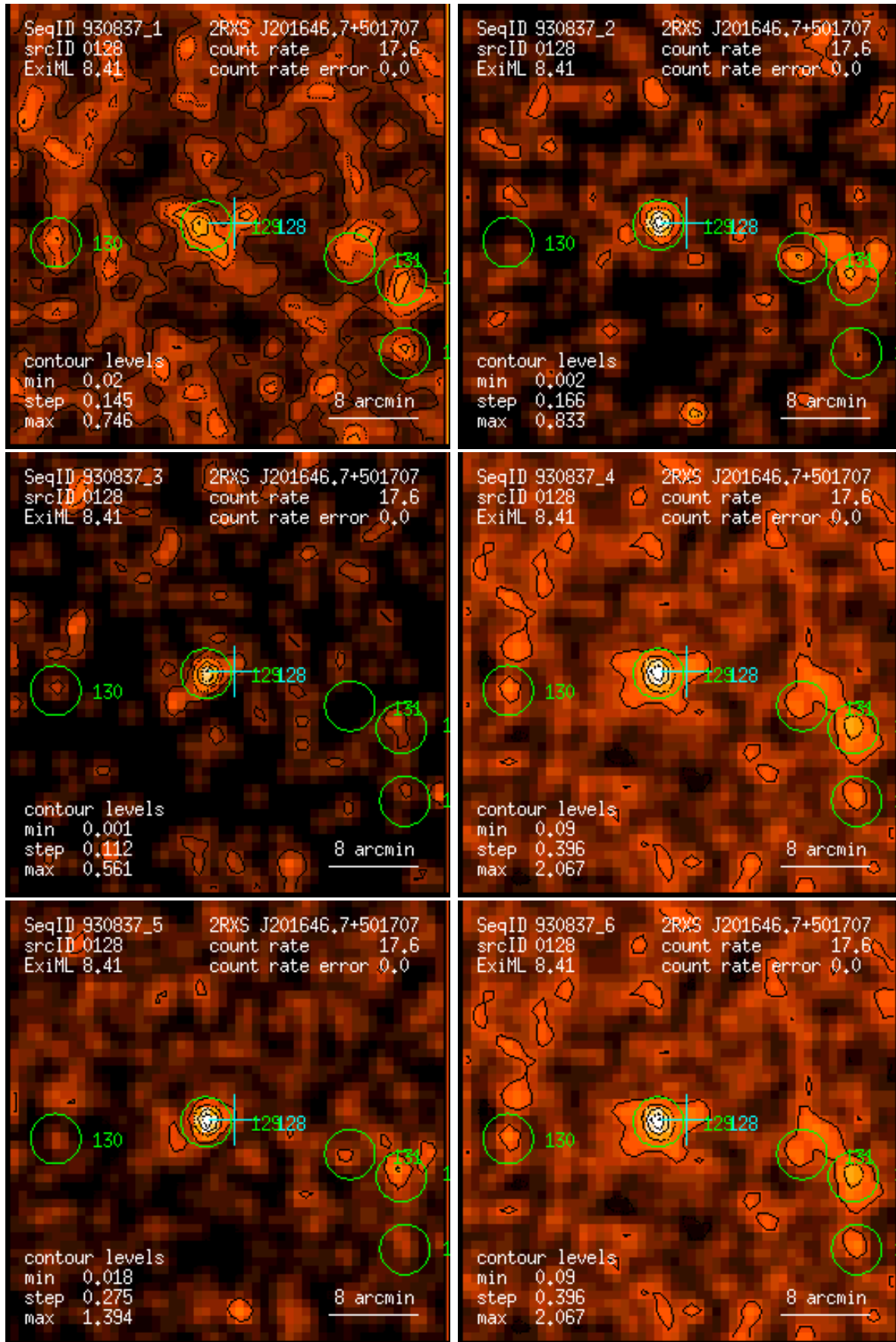
Figure 128: RASS 930837: detection 0128: band rate images, Gaussian filter: (1) PSPC channels 11 – 41, (2) 52 – 90, (3) 91 – 201, (4) 11 – 235, (5) 52 – 201, (6) 11 – 201. Broad band rates in counts/ks. Band rate contour levels in counts/ks/arcmin 2 .
