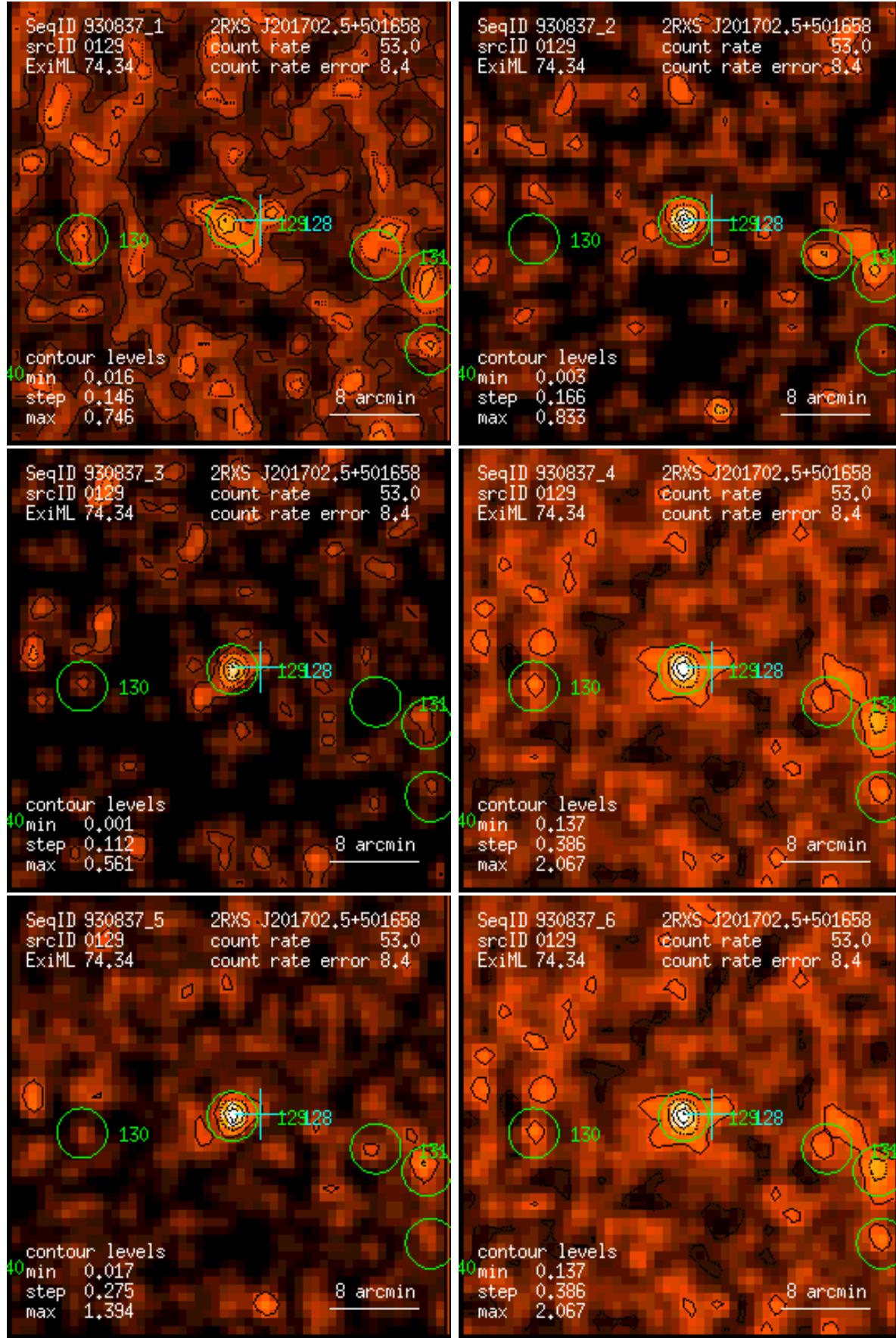
Figure 129: RASS 930837: detection 0129: band rate images, Gaussian filter: (1) PSPC channels 11 – 41, (2) 52 – 90, (3) 91 – 201, (4) 11 – 235, (5) 52 – 201, (6) 11 – 201. Broad band rates in counts/ks. Band rate contour levels in counts/ks/arcmin 2 .
