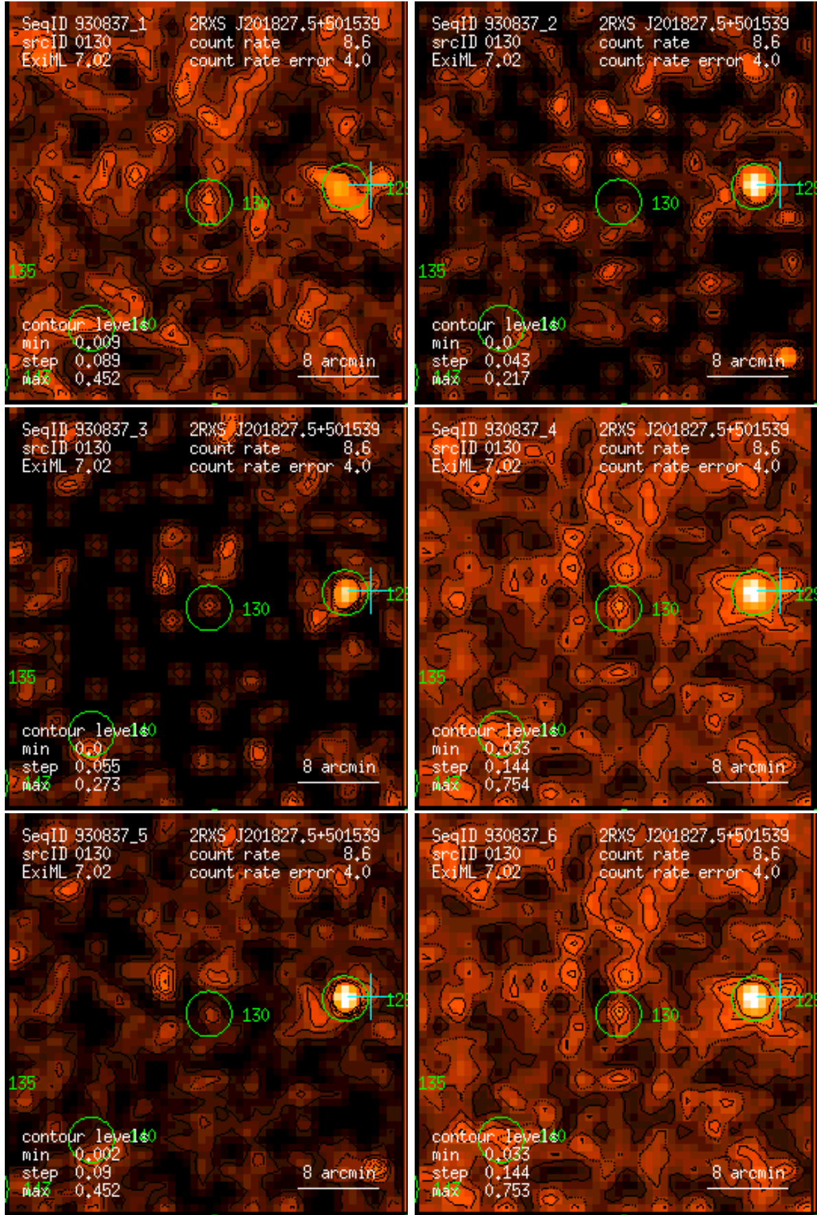
Figure 130: RASS 930837: detection 0130: band rate images, Gaussian filter: (1) PSPC channels 11 – 41, (2) 52 – 90, (3) 91 – 201, (4) 11 – 235, (5) 52 – 201, (6) 11 – 201. Broad band rates in counts/ks. Band rate contour levels in counts/ks/arcmin 2 .
