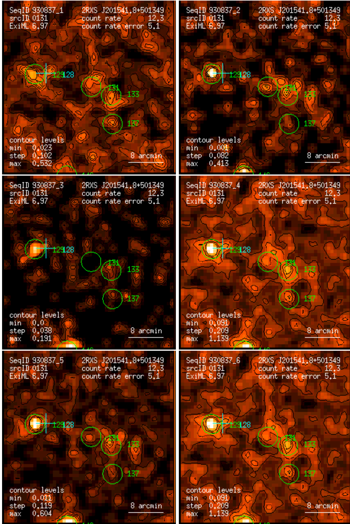
Figure 131: RASS 930837: detection 0131: band rate images, Gaussian filter: (1) PSPC channels 11 – 41, (2) 52 – 90, (3) 91 – 201, (4) 11 – 235, (5) 52 – 201, (6) 11 – 201. Broad band rates in counts/ks. Band rate contour levels in counts/ks/arcmin 2 .
