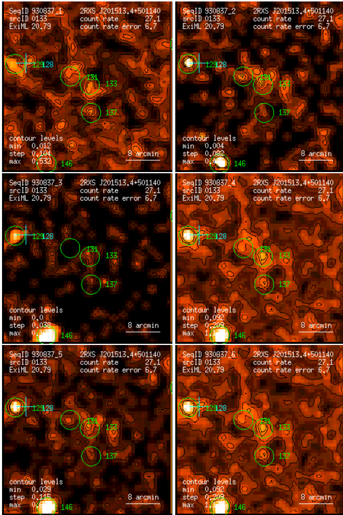
Figure 133: RASS 930837: detection 0133: band rate images, Gaussian filter: (1) PSPC channels 11 – 41, (2) 52 – 90, (3) 91 – 201, (4) 11 – 235, (5) 52 – 201, (6) 11 – 201. Broad band rates in counts/ks. Band rate contour levels in counts/ks/arcmin 2 .
