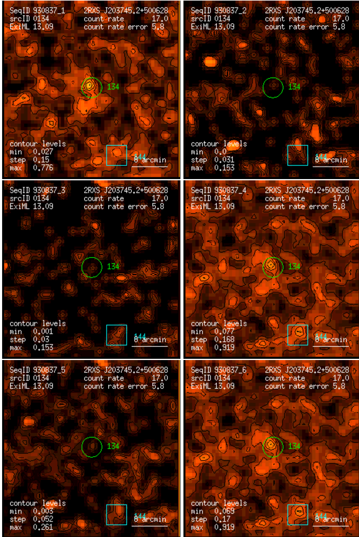
Figure 134: RASS 930837: detection 0134: band rate images, Gaussian filter: (1) PSPC channels 11 – 41, (2) 52 – 90, (3) 91 – 201, (4) 11 – 235, (5) 52 – 201, (6) 11 – 201. Broad band rates in counts/ks. Band rate contour levels in counts/ks/arcmin 2 .
