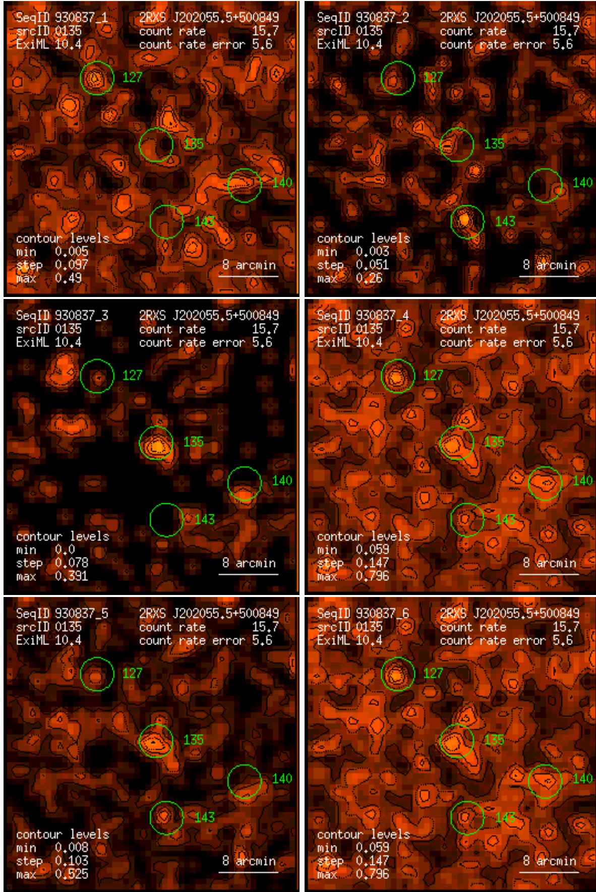
Figure 135: RASS 930837: detection 0135: band rate images, Gaussian filter: (1) PSPC channels 11 – 41, (2) 52 – 90, (3) 91 – 201, (4) 11 – 235, (5) 52 – 201, (6) 11 – 201. Broad band rates in counts/ks. Band rate contour levels in counts/ks/arcmin 2 .
