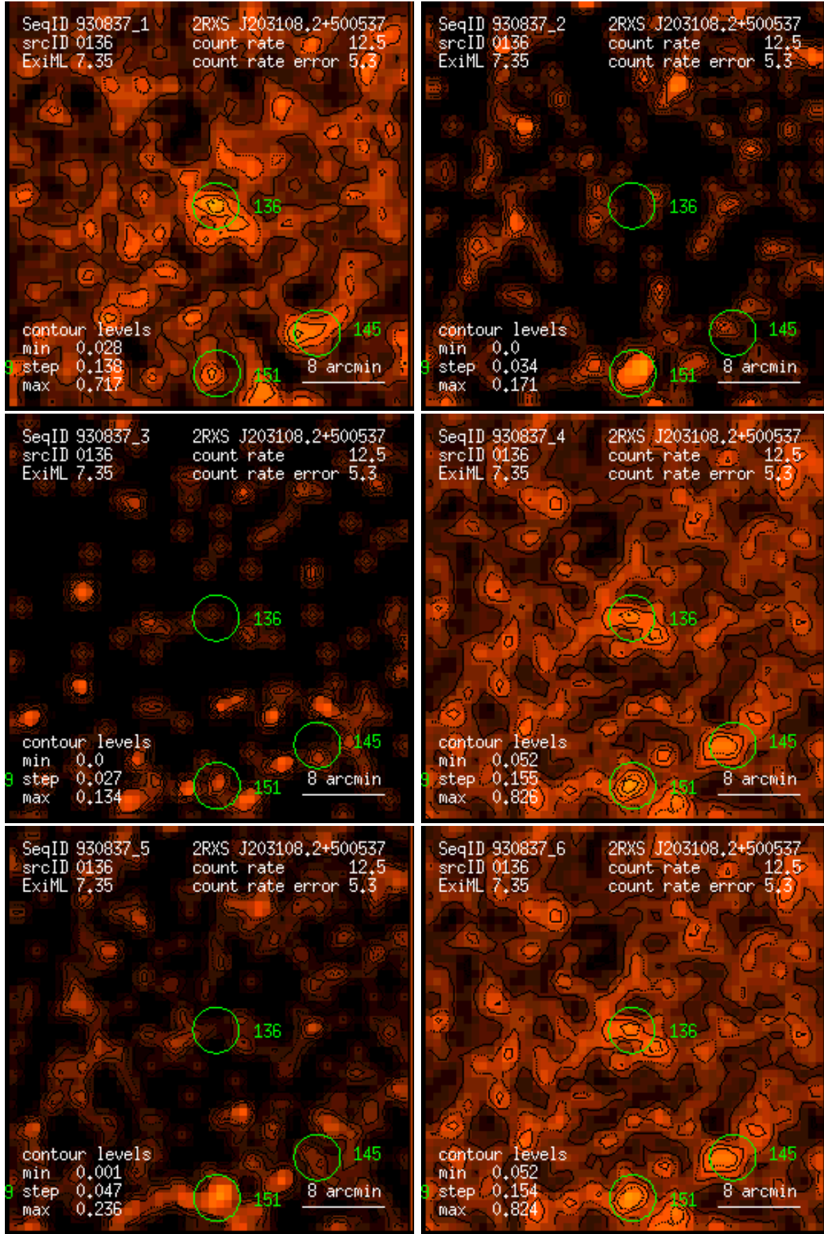
Figure 136: RASS 930837: detection 0136: band rate images, Gaussian filter: (1) PSPC channels 11 – 41, (2) 52 – 90, (3) 91 – 201, (4) 11 – 235, (5) 52 – 201, (6) 11 – 201. Broad band rates in counts/ks. Band rate contour levels in counts/ks/arcmin 2 .
