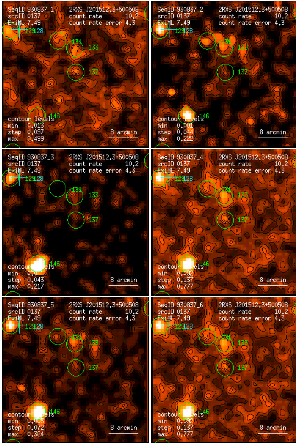
Figure 137: RASS 930837: detection 0137: band rate images, Gaussian filter: (1) PSPC channels 11 – 41, (2) 52 – 90, (3) 91 – 201, (4) 11 – 235, (5) 52 – 201, (6) 11 – 201. Broad band rates in counts/ks. Band rate contour levels in counts/ks/arcmin 2 .
