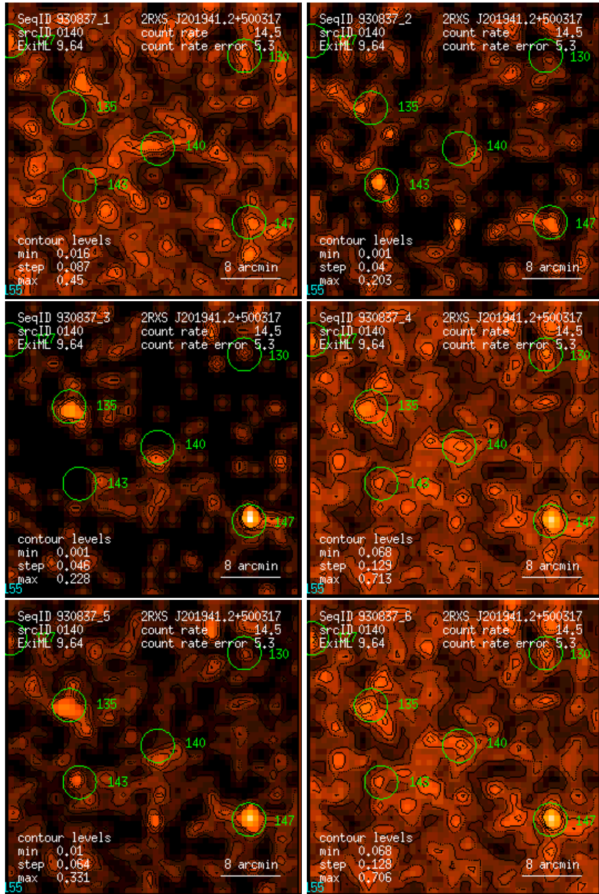
Figure 140: RASS 930837: detection 0140: band rate images, Gaussian filter: (1) PSPC channels 11 – 41, (2) 52 – 90, (3) 91 – 201, (4) 11 – 235, (5) 52 – 201, (6) 11 – 201. Broad band rates in counts/ks. Band rate contour levels in counts/ks/arcmin 2 .
