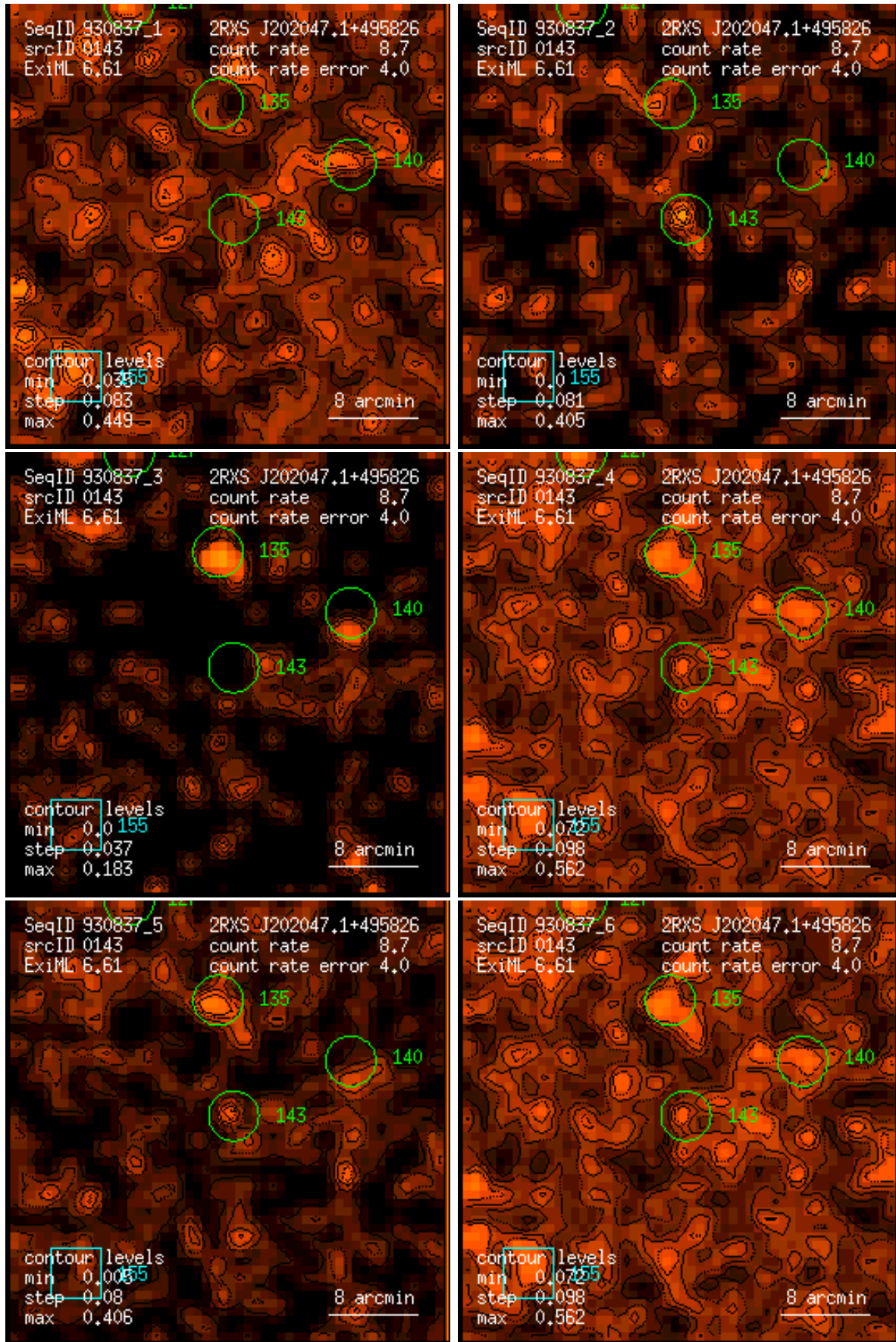
Figure 143: RASS 930837: detection 0143: band rate images, Gaussian filter: (1) PSPC channels 11 – 41, (2) 52 – 90, (3) 91 – 201, (4) 11 – 235, (5) 52 – 201, (6) 11 – 201. Broad band rates in counts/ks. Band rate contour levels in counts/ks/arcmin 2 .
