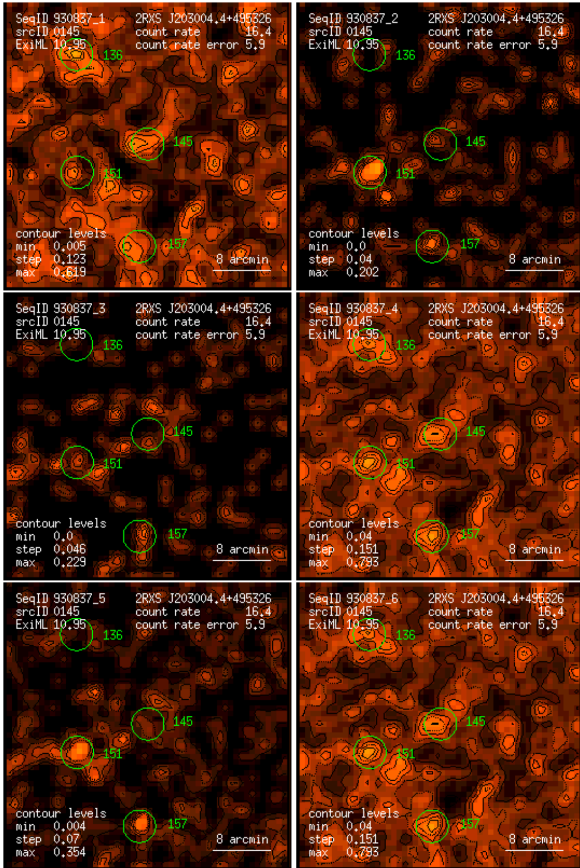
Figure 145: RASS 930837: detection 0145: band rate images, Gaussian filter: (1) PSPC channels 11 – 41, (2) 52 – 90, (3) 91 – 201, (4) 11 – 235, (5) 52 – 201, (6) 11 – 201. Broad band rates in counts/ks. Band rate contour levels in counts/ks/arcmin 2 .
