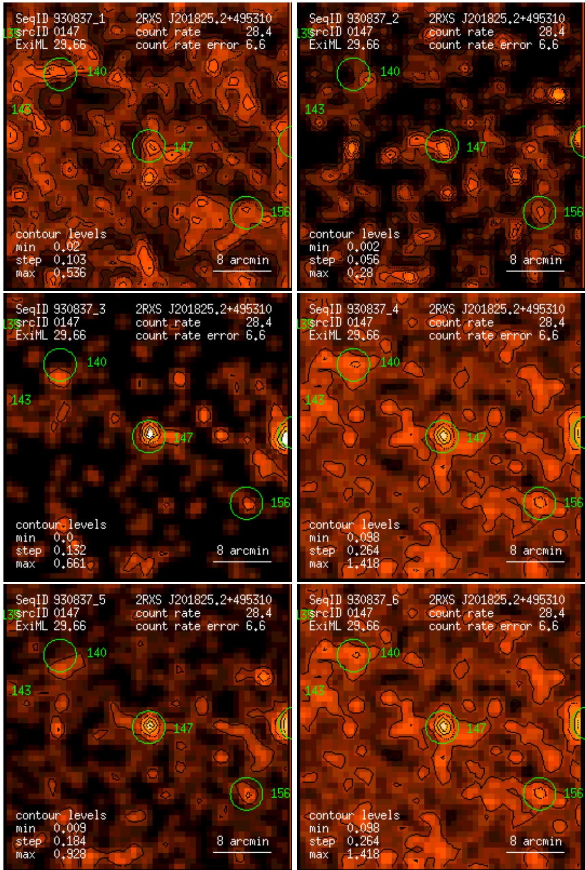
Figure 147: RASS 930837: detection 0147: band rate images, Gaussian filter: (1) PSPC channels 11 – 41, (2) 52 – 90, (3) 91 – 201, (4) 11 – 235, (5) 52 – 201, (6) 11 – 201. Broad band rates in counts/ks. Band rate contour levels in counts/ks/arcmin 2 .
