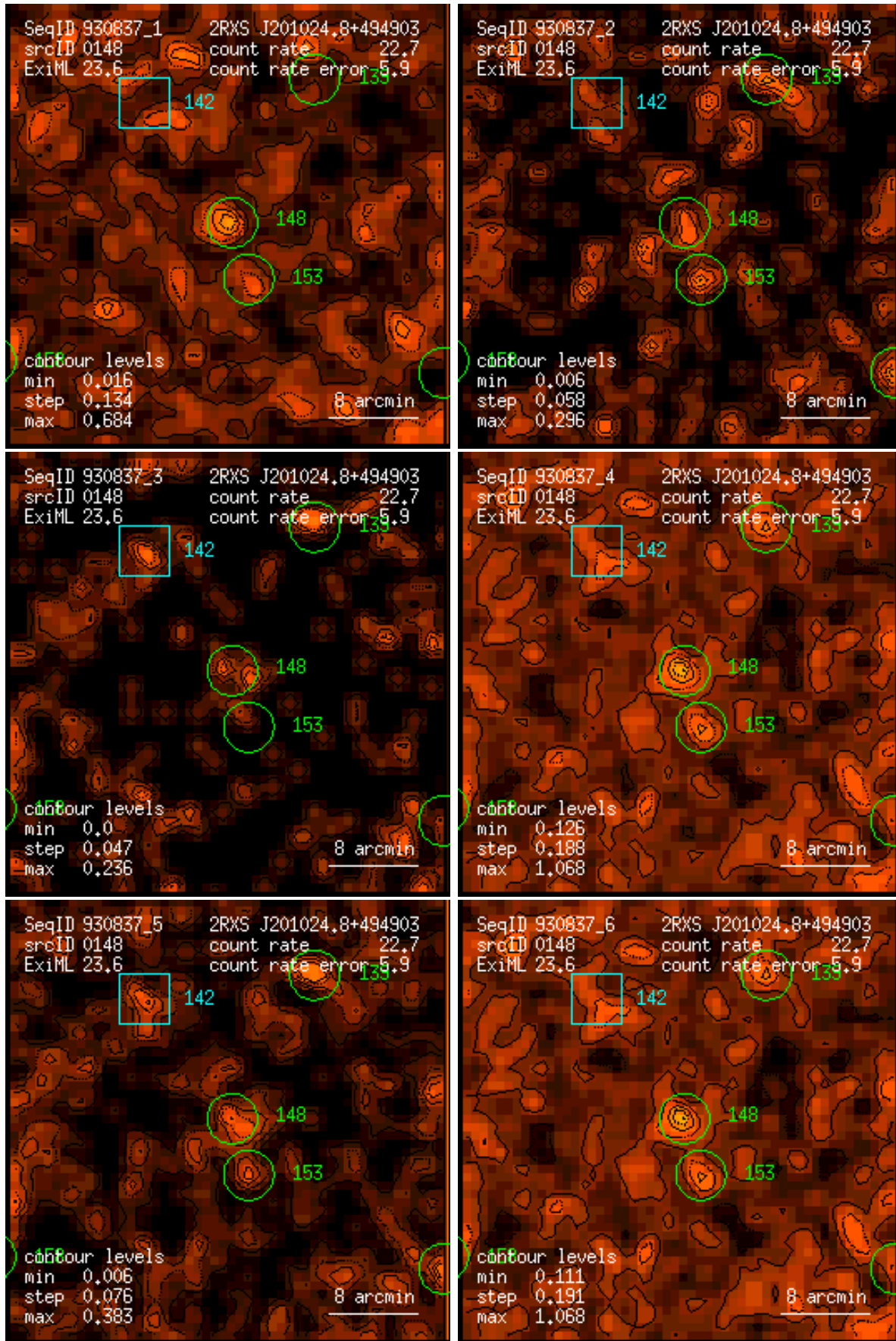
Figure 148: RASS 930837: detection 0148: band rate images, Gaussian filter: (1) PSPC channels 11 – 41, (2) 52 – 90, (3) 91 – 201, (4) 11 – 235, (5) 52 – 201, (6) 11 – 201. Broad band rates in counts/ks. Band rate contour levels in counts/ks/arcmin 2 .
