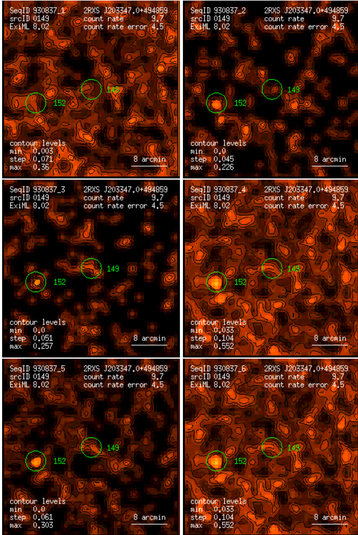
Figure 149: RASS 930837: detection 0149: band rate images, Gaussian filter: (1) PSPC channels 11 – 41, (2) 52 – 90, (3) 91 – 201, (4) 11 – 235, (5) 52 – 201, (6) 11 – 201. Broad band rates in counts/ks. Band rate contour levels in counts/ks/arcmin 2 .
