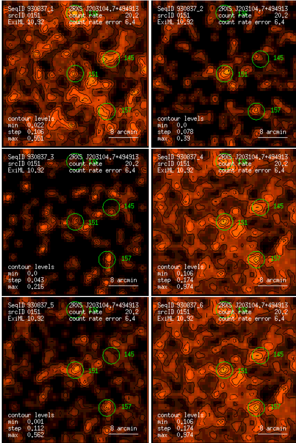
Figure 151: RASS 930837: detection 0151: band rate images, Gaussian filter: (1) PSPC channels 11 – 41, (2) 52 – 90, (3) 91 – 201, (4) 11 – 235, (5) 52 – 201, (6) 11 – 201. Broad band rates in counts/ks. Band rate contour levels in counts/ks/arcmin 2 .
