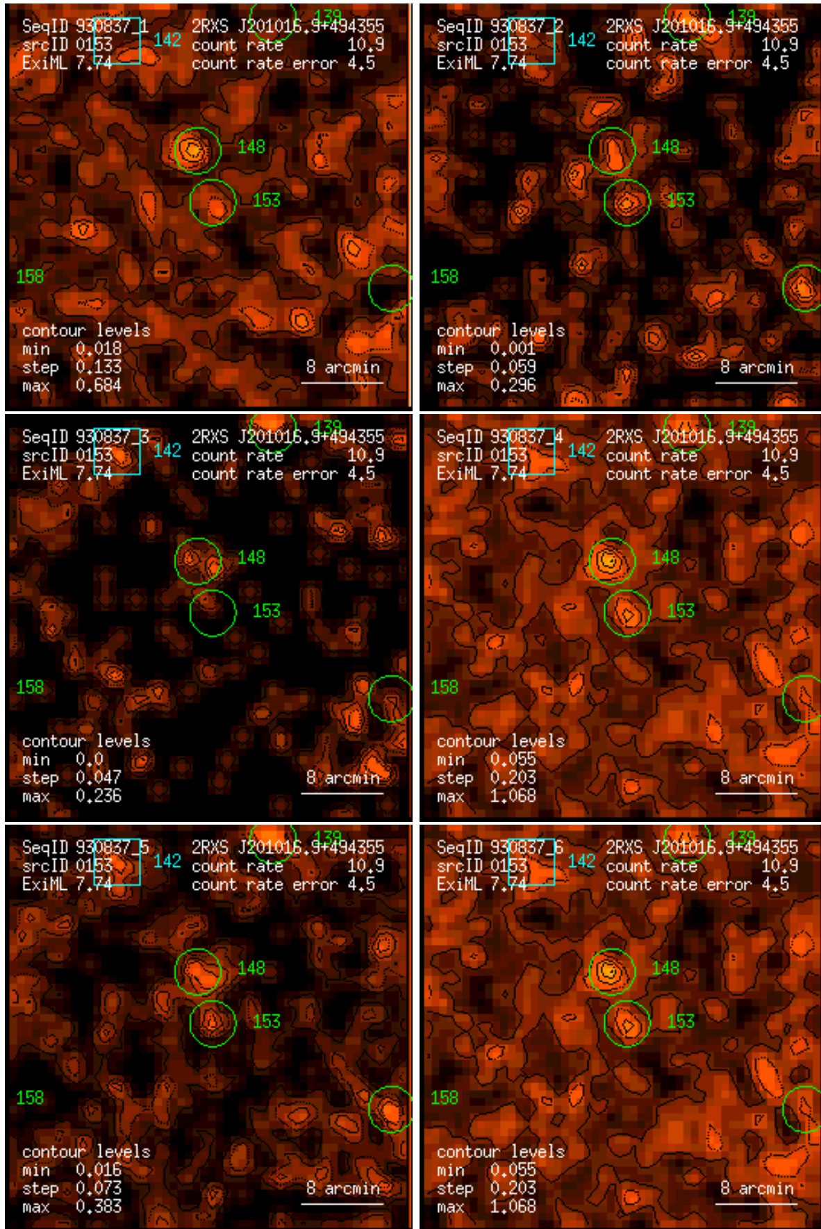
Figure 153: RASS 930837: detection 0153: band rate images, Gaussian filter: (1) PSPC channels 11 – 41, (2) 52 – 90, (3) 91 – 201, (4) 11 – 235, (5) 52 – 201, (6) 11 – 201. Broad band rates in counts/ks. Band rate contour levels in counts/ks/arcmin 2 .
