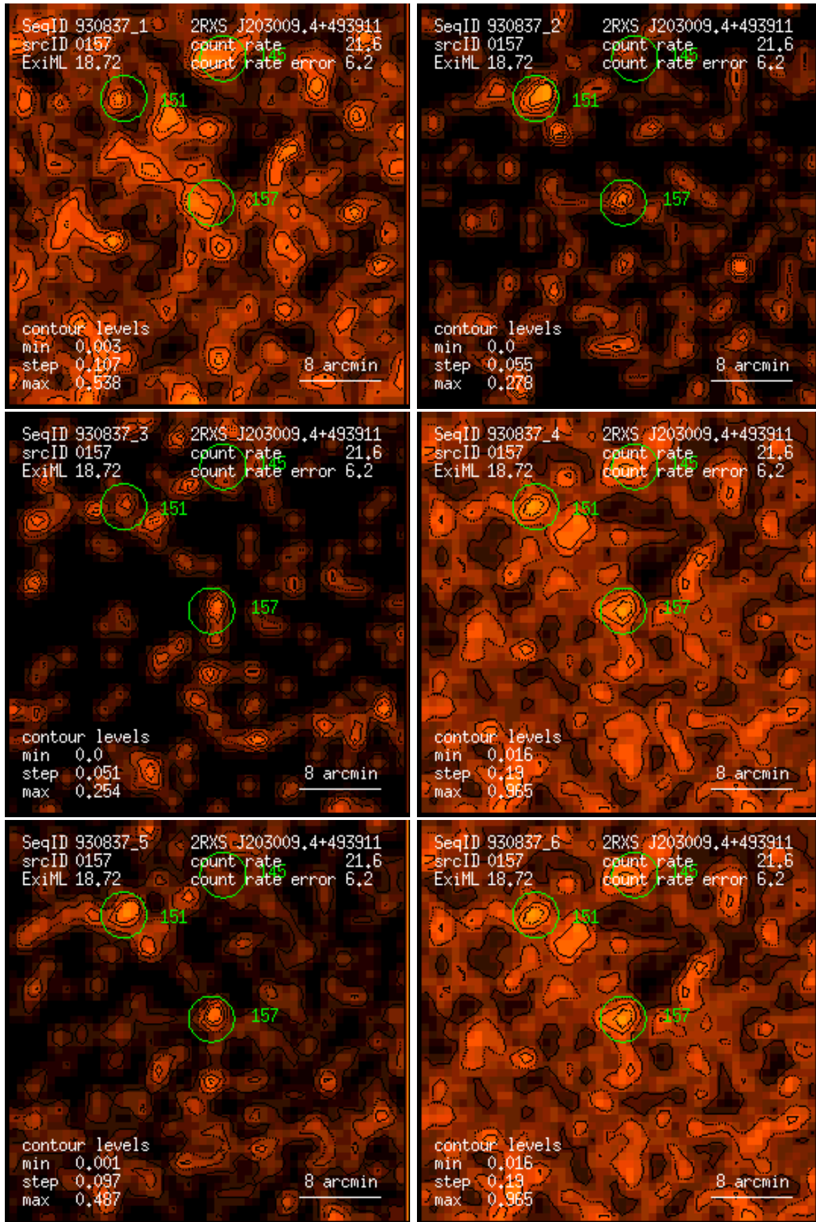
Figure 157: RASS 930837: detection 0157: band rate images, Gaussian filter: (1) PSPC channels 11 – 41, (2) 52 – 90, (3) 91 – 201, (4) 11 – 235, (5) 52 – 201, (6) 11 – 201. Broad band rates in counts/ks. Band rate contour levels in counts/ks/arcmin 2 .
