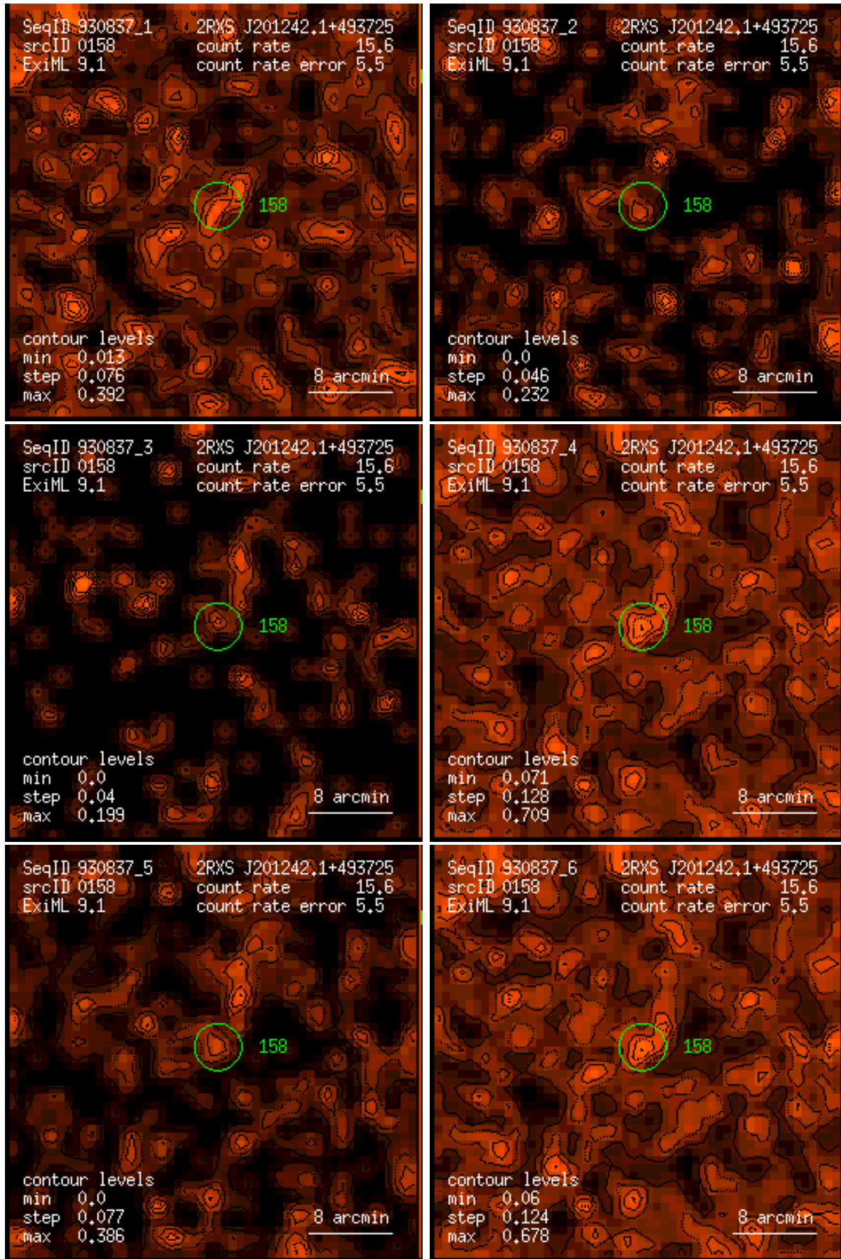
Figure 158: RASS 930837: detection 0158: band rate images, Gaussian filter: (1) PSPC channels 11 – 41, (2) 52 – 90, (3) 91 – 201, (4) 11 – 235, (5) 52 – 201, (6) 11 – 201. Broad band rates in counts/ks. Band rate contour levels in counts/ks/arcmin 2 .
